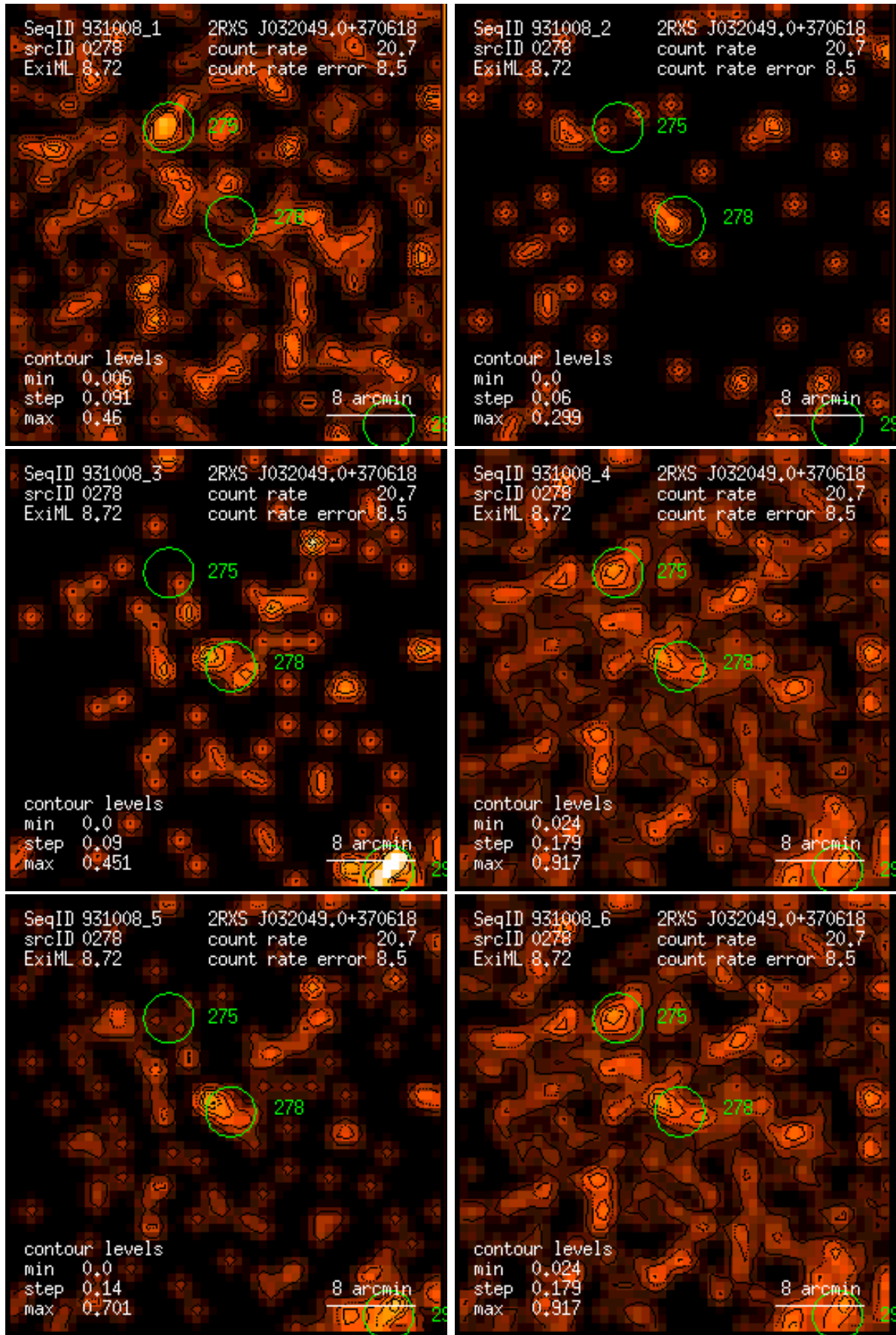
Figure 278: RASS 931008: detection 0278: band rate images, Gaussian filter: (1) PSPC channels 11 – 41, (2) 52 – 90, (3) 91 – 201, (4) 11 – 235, (5) 52 – 201, (6) 11 – 201. Broad band rates in counts/ks. Band rate contour levels in counts/ks/arcmin 2 .
