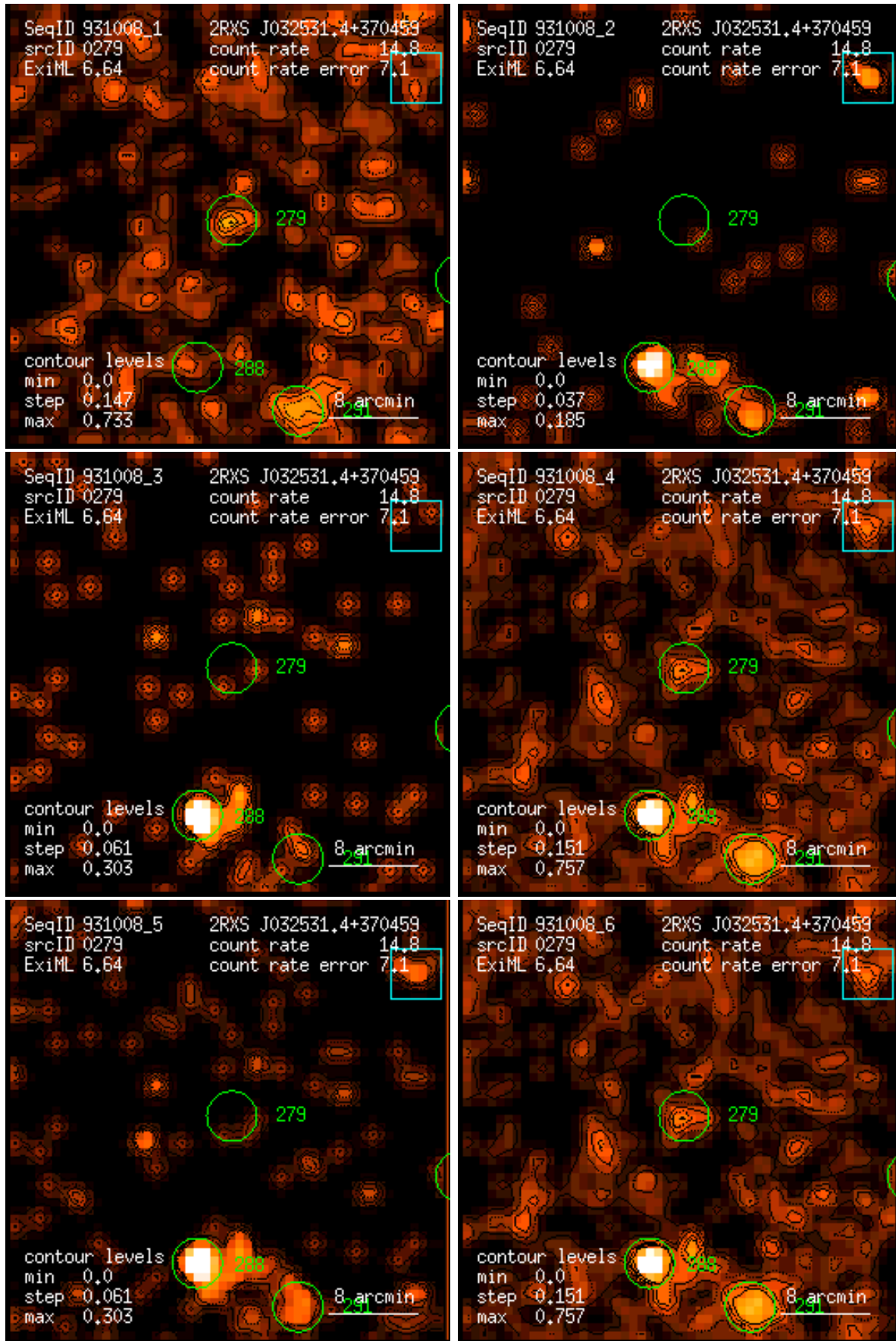
Figure 279: RASS 931008: detection 0279: band rate images, Gaussian filter: (1) PSPC channels 11 – 41, (2) 52 – 90, (3) 91 – 201, (4) 11 – 235, (5) 52 – 201, (6) 11 – 201. Broad band rates in counts/ks. Band rate contour levels in counts/ks/arcmin 2 .
