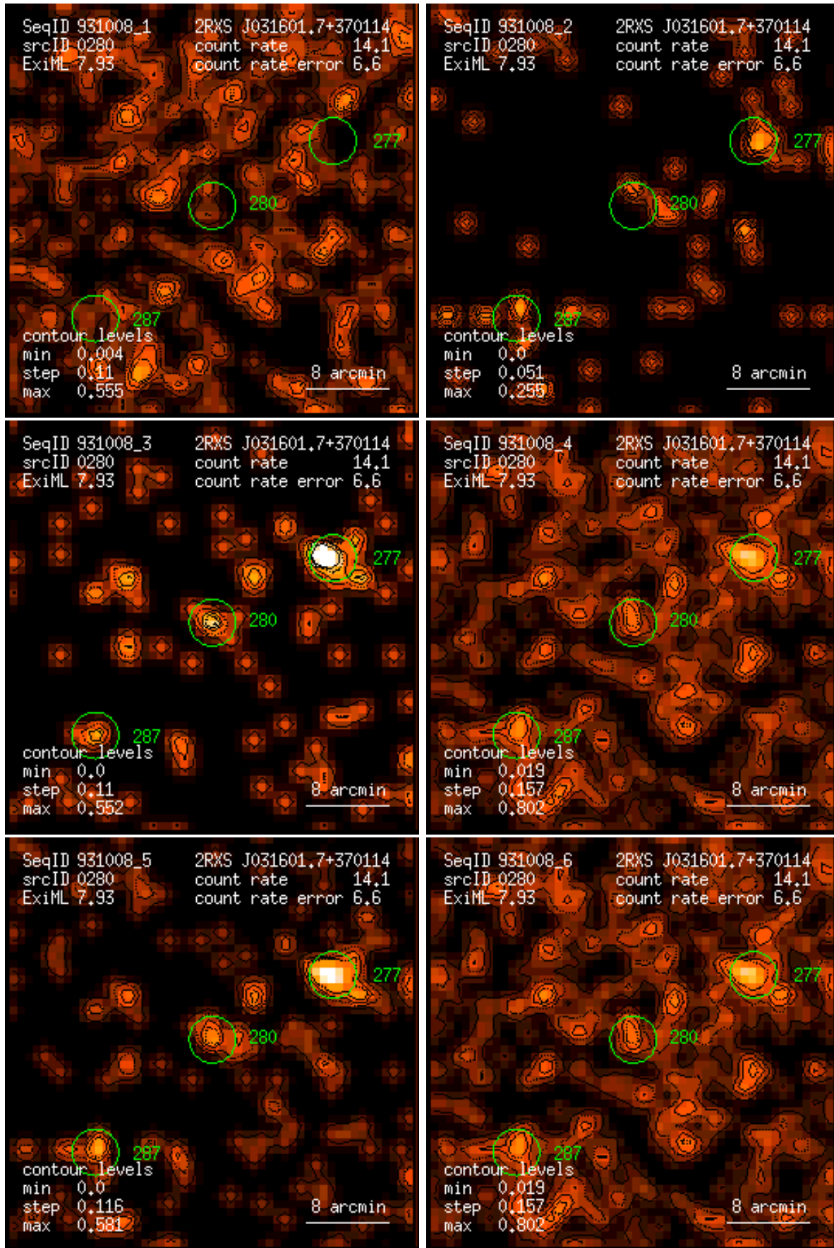
Figure 280: RASS 931008: detection 0280: band rate images, Gaussian filter: (1) PSPC channels 11 – 41, (2) 52 – 90, (3) 91 – 201, (4) 11 – 235, (5) 52 – 201, (6) 11 – 201. Broad band rates in counts/ks. Band rate contour levels in counts/ks/arcmin 2 .
