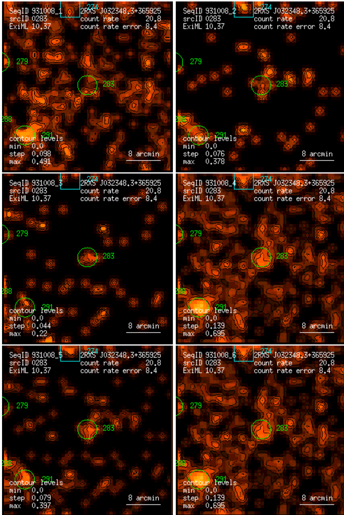
Figure 283: RASS 931008: detection 0283: band rate images, Gaussian filter: (1) PSPC channels 11 – 41, (2) 52 – 90, (3) 91 – 201, (4) 11 – 235, (5) 52 – 201, (6) 11 – 201. Broad band rates in counts/ks. Band rate contour levels in counts/ks/arcmin 2 .
