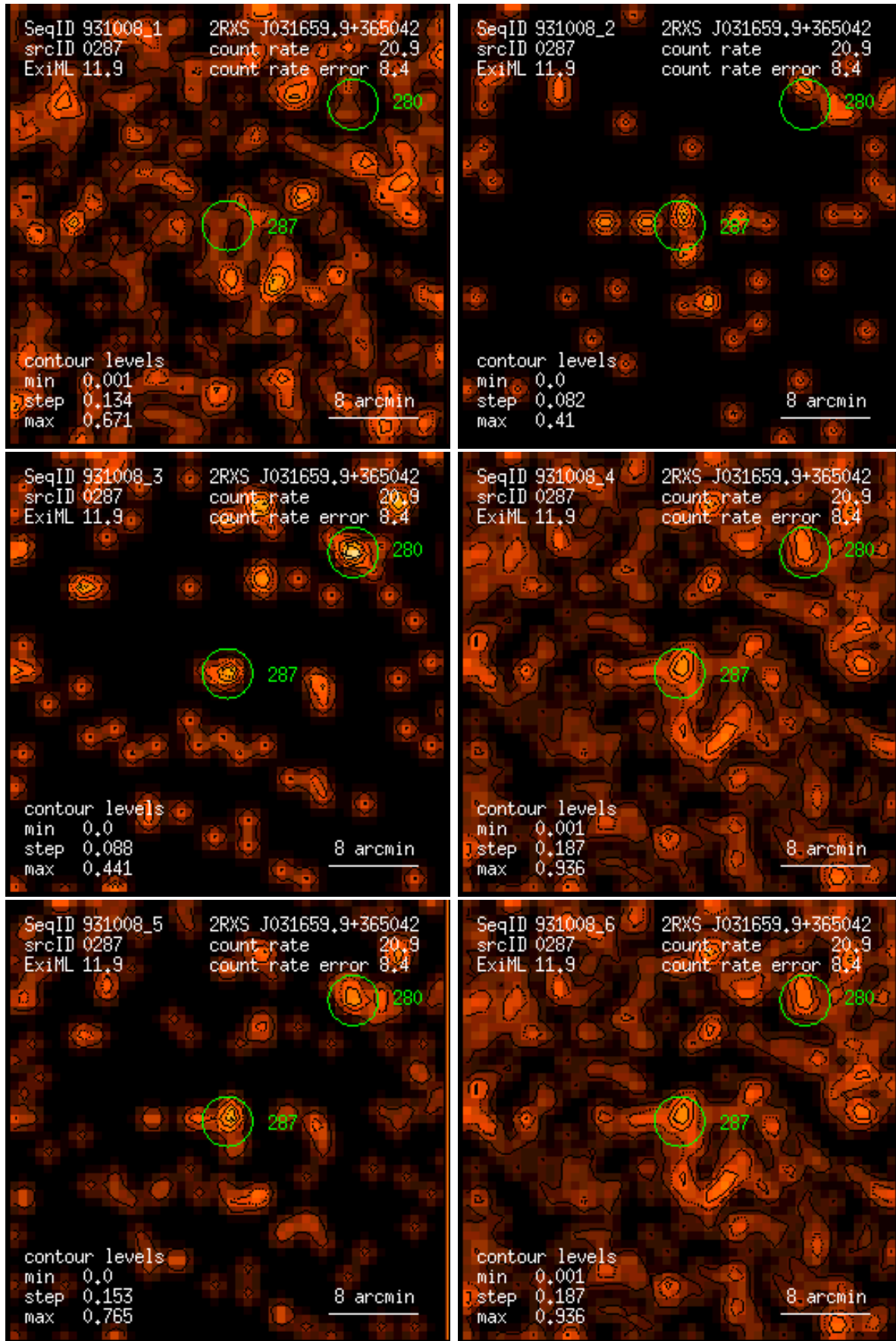
Figure 287: RASS 931008: detection 0287: band rate images, Gaussian filter: (1) PSPC channels 11 – 41, (2) 52 – 90, (3) 91 – 201, (4) 11 – 235, (5) 52 – 201, (6) 11 – 201. Broad band rates in counts/ks. Band rate contour levels in counts/ks/arcmin 2 .
