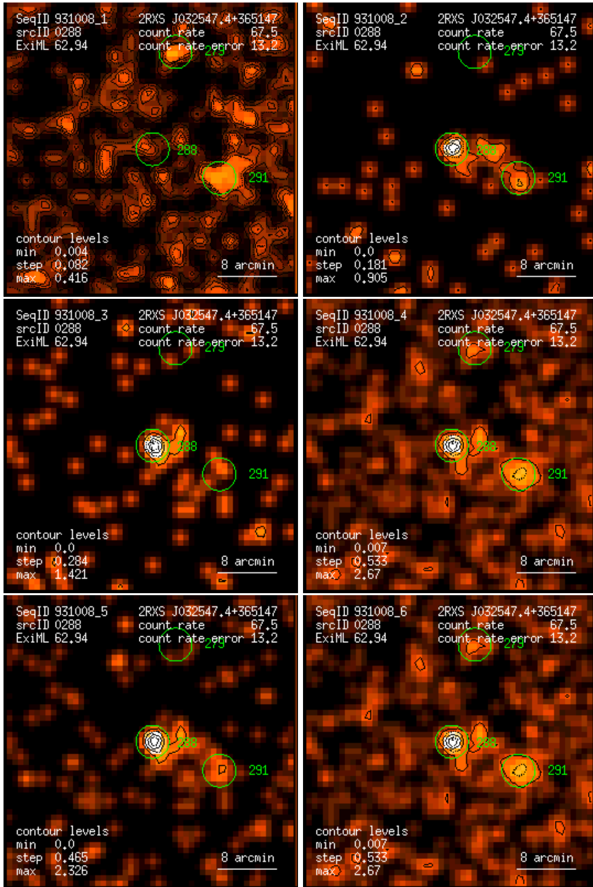
Figure 288: RASS 931008: detection 0288: band rate images, Gaussian filter: (1) PSPC channels 11 – 41, (2) 52 – 90, (3) 91 – 201, (4) 11 – 235, (5) 52 – 201, (6) 11 – 201. Broad band rates in counts/ks. Band rate contour levels in counts/ks/arcmin 2 .
