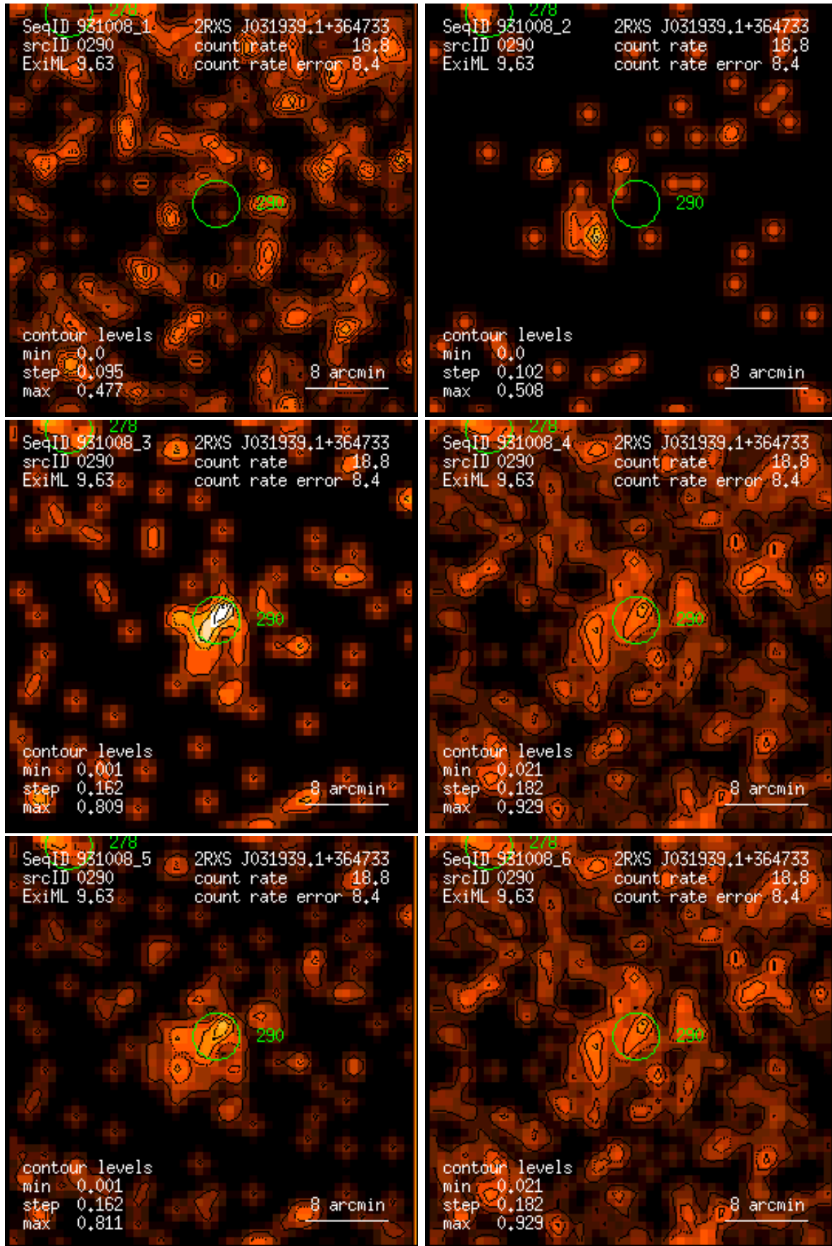
Figure 290: RASS 931008: detection 0290: band rate images, Gaussian filter: (1) PSPC channels 11 – 41, (2) 52 – 90, (3) 91 – 201, (4) 11 – 235, (5) 52 – 201, (6) 11 – 201. Broad band rates in counts/ks. Band rate contour levels in counts/ks/arcmin 2 .
