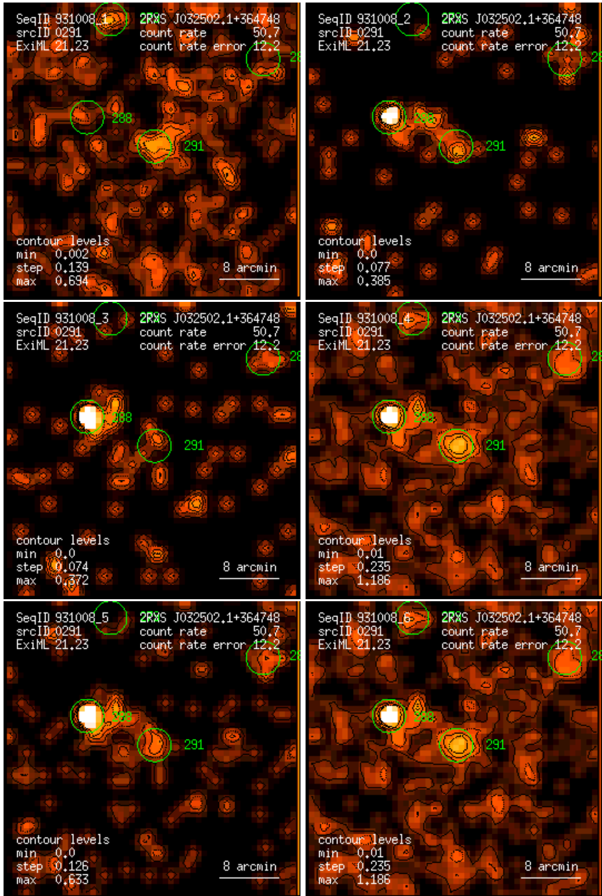
Figure 291: RASS 931008: detection 0291: band rate images, Gaussian filter: (1) PSPC channels 11 – 41, (2) 52 – 90, (3) 91 – 201, (4) 11 – 235, (5) 52 – 201, (6) 11 – 201. Broad band rates in counts/ks. Band rate contour levels in counts/ks/arcmin 2 .
