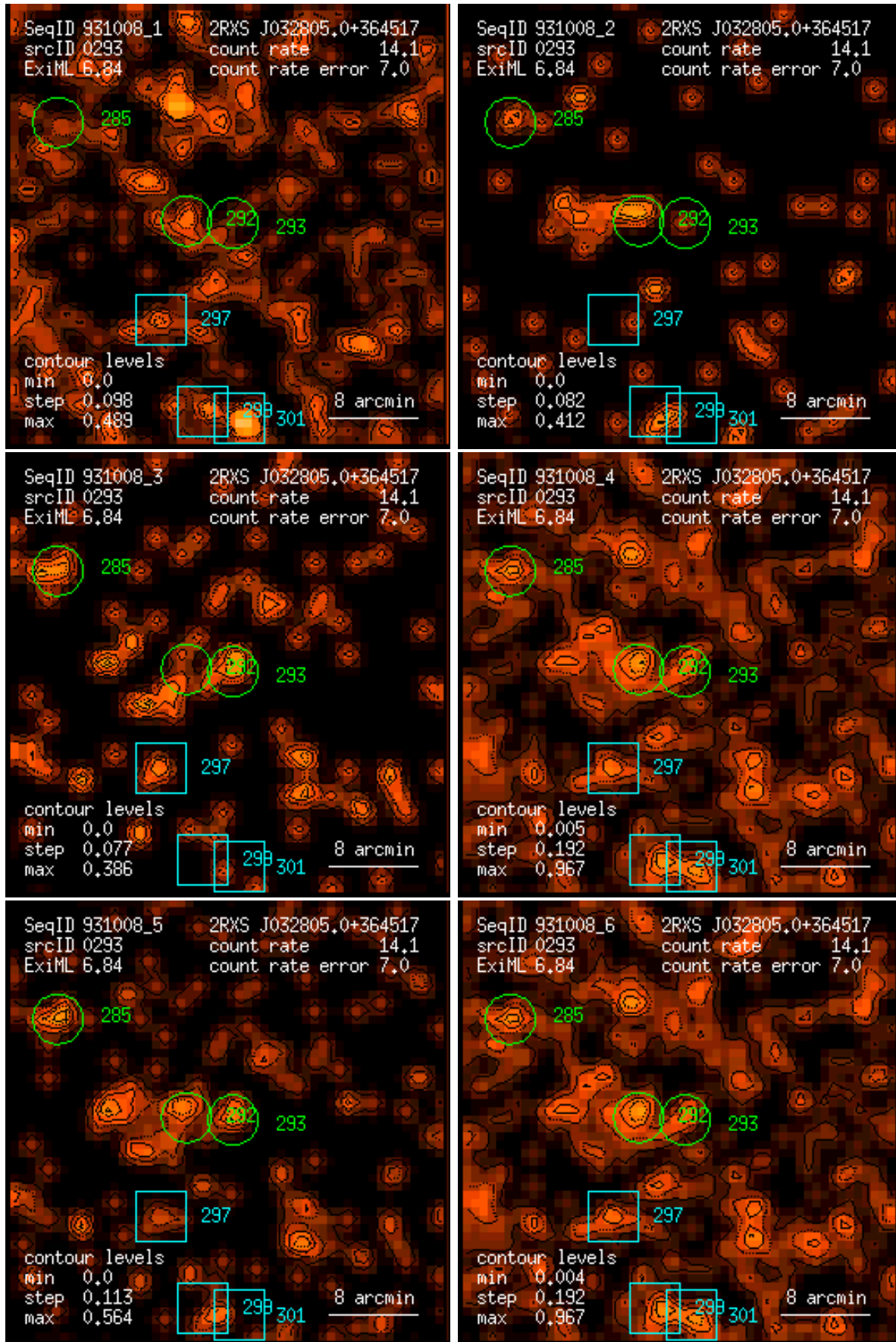
Figure 293: RASS 931008: detection 0293: band rate images, Gaussian filter: (1) PSPC channels 11 – 41, (2) 52 – 90, (3) 91 – 201, (4) 11 – 235, (5) 52 – 201, (6) 11 – 201. Broad band rates in counts/ks. Band rate contour levels in counts/ks/arcmin 2 .
