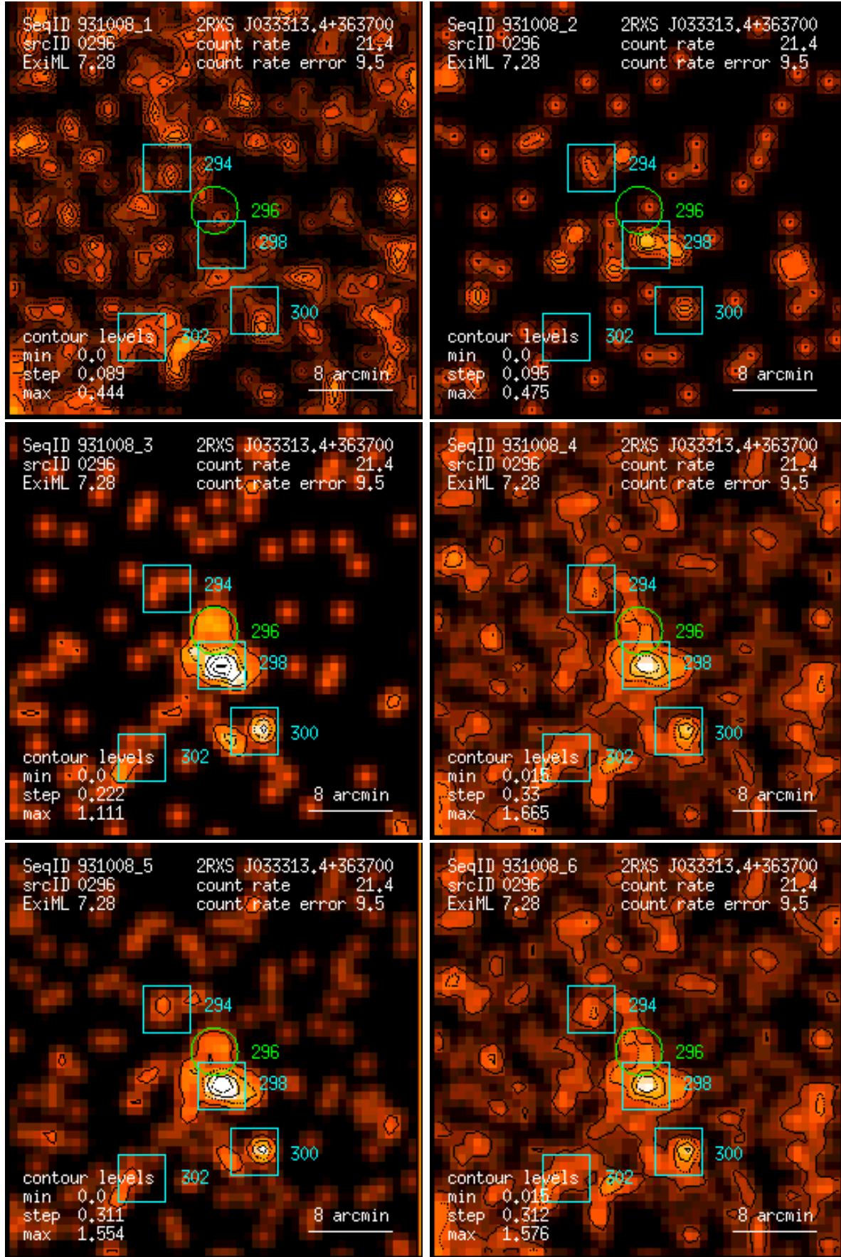
Figure 296: RASS 931008: detection 0296: band rate images, Gaussian filter: (1) PSPC channels 11 – 41, (2) 52 – 90, (3) 91 – 201, (4) 11 – 235, (5) 52 – 201, (6) 11 – 201. Broad band rates in counts/ks. Band rate contour levels in counts/ks/arcmin 2 .
