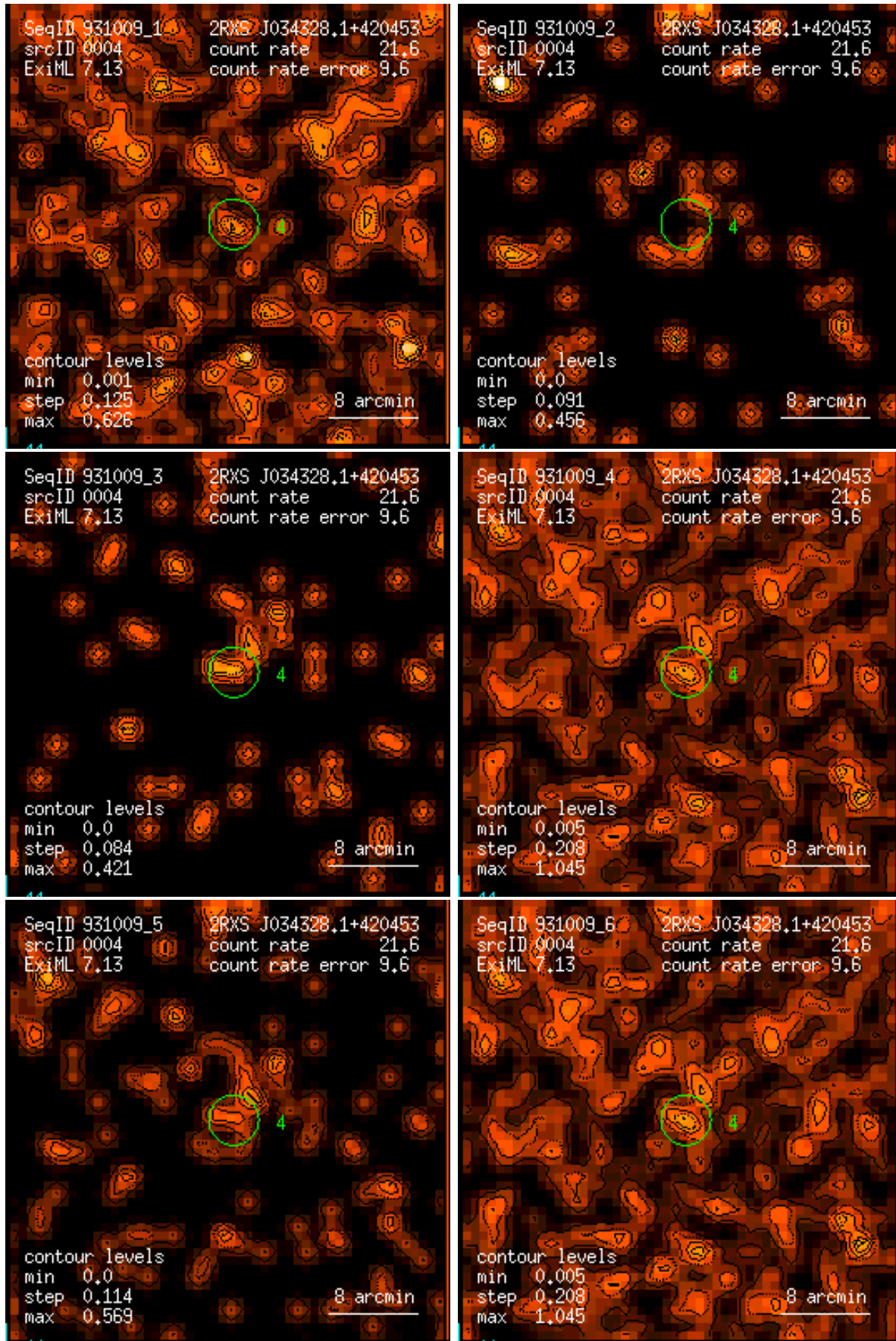
Figure 4: RASS 931009: detection 0004: band rate images, Gaussian filter: (1) PSPC channels 11 – 41, (2) 52 – 90, (3) 91 – 201, (4) 11 – 235, (5) 52 – 201, (6) 11 – 201. Broad band rates in counts/ks. Band rate contour levels in counts/ks/arcmin 2 .
