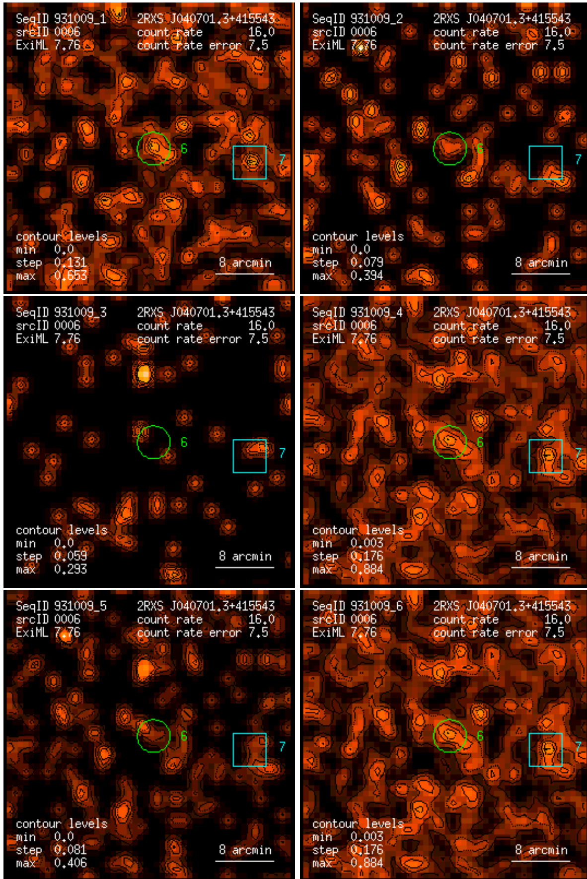
Figure 6: RASS 931009: detection 0006: band rate images, Gaussian filter: (1) PSPC channels 11 – 41, (2) 52 – 90, (3) 91 – 201, (4) 11 – 235, (5) 52 – 201, (6) 11 – 201. Broad band rates in counts/ks. Band rate contour levels in counts/ks/arcmin 2 .
