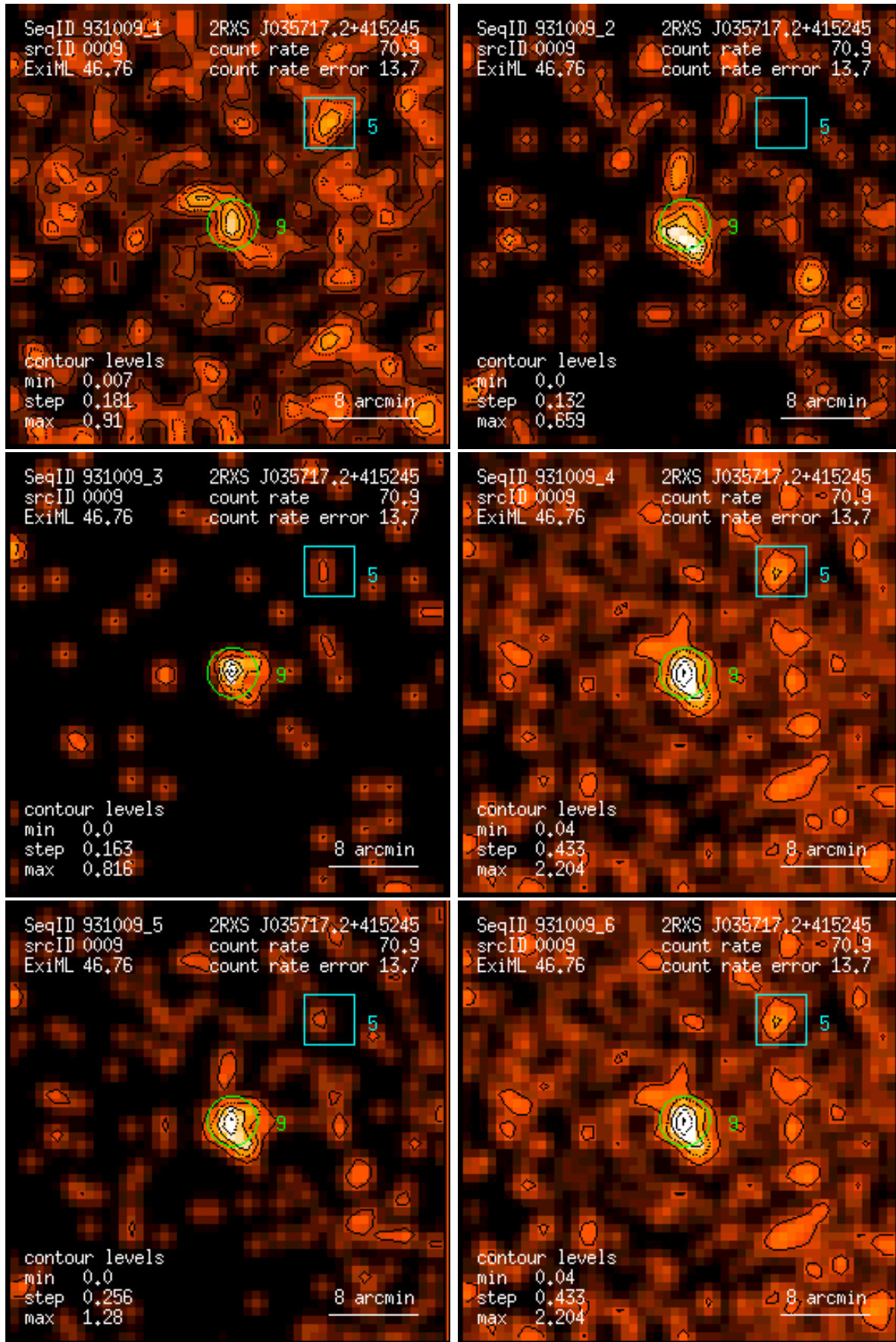
Figure 9: RASS 931009: detection 0009: band rate images, Gaussian filter: (1) PSPC channels 11 – 41, (2) 52 – 90, (3) 91 – 201, (4) 11 – 235, (5) 52 – 201, (6) 11 – 201. Broad band rates in counts/ks. Band rate contour levels in counts/ks/arcmin 2 .
