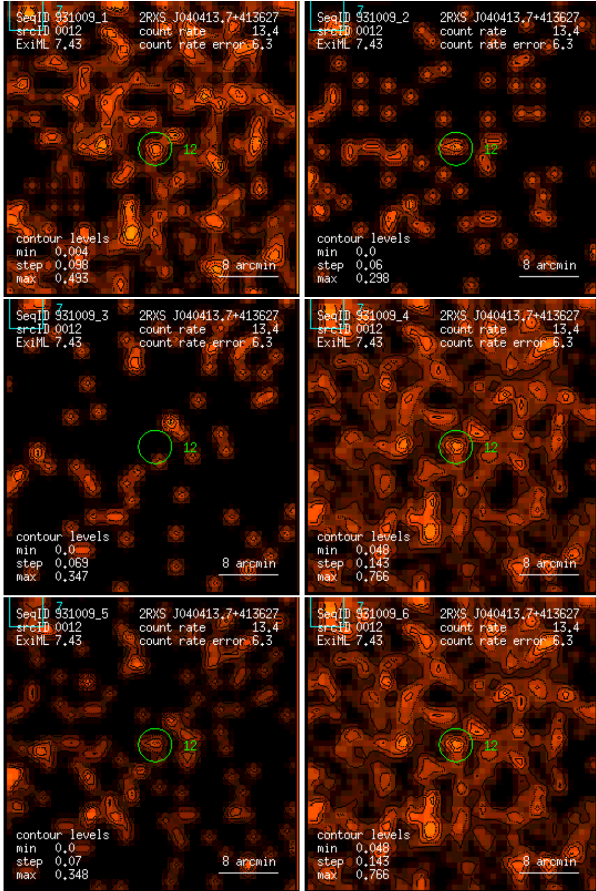
Figure 12: RASS 931009: detection 0012: band rate images, Gaussian filter: (1) PSPC channels 11 – 41, (2) 52 – 90, (3) 91 – 201, (4) 11 – 235, (5) 52 – 201, (6) 11 – 201. Broad band rates in counts/ks. Band rate contour levels in counts/ks/arcmin 2 .
