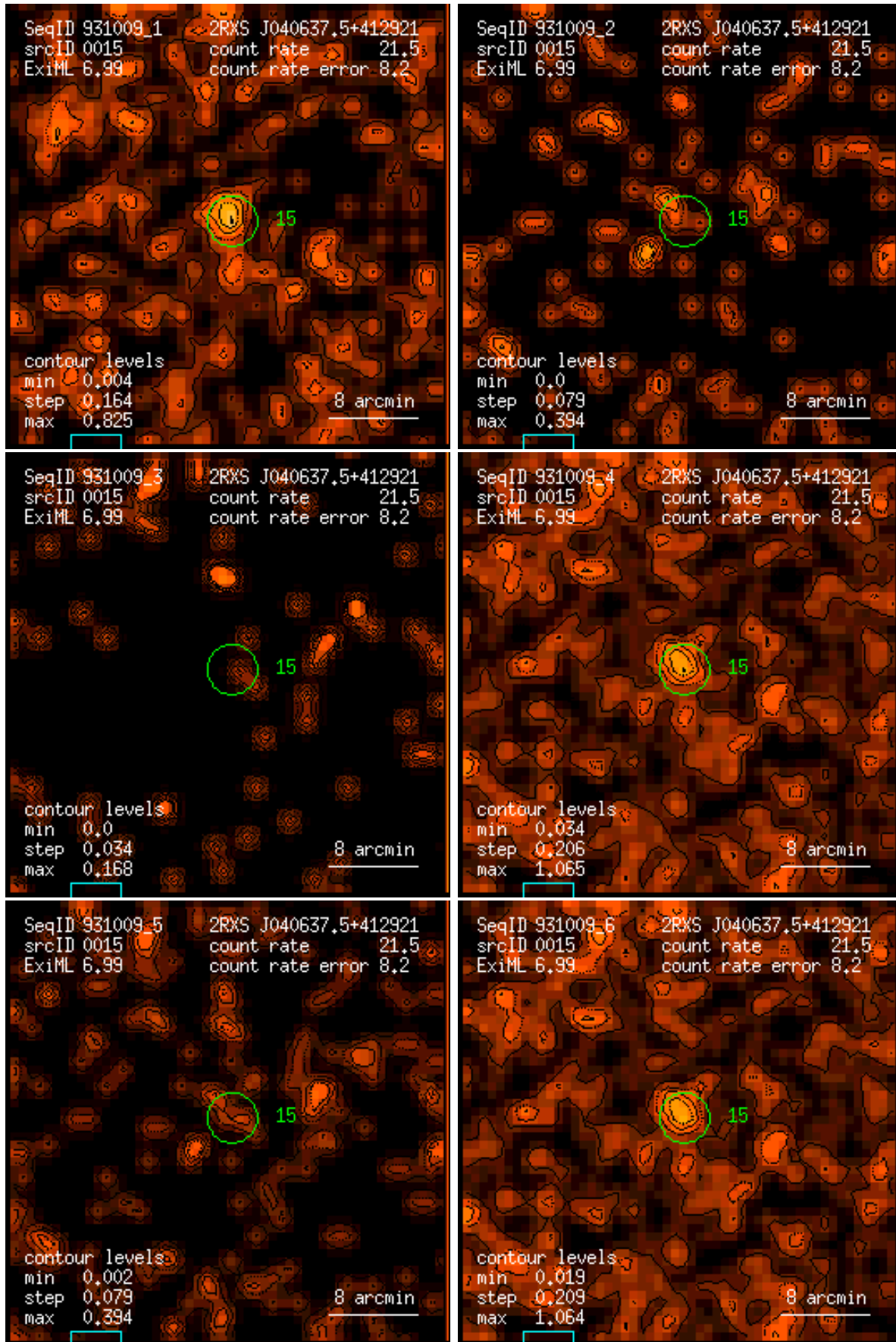
Figure 15: RASS 931009: detection 0015: band rate images, Gaussian filter: (1) PSPC channels 11 – 41, (2) 52 – 90, (3) 91 – 201, (4) 11 – 235, (5) 52 – 201, (6) 11 – 201. Broad band rates in counts/ks. Band rate contour levels in counts/ks/arcmin 2 .
