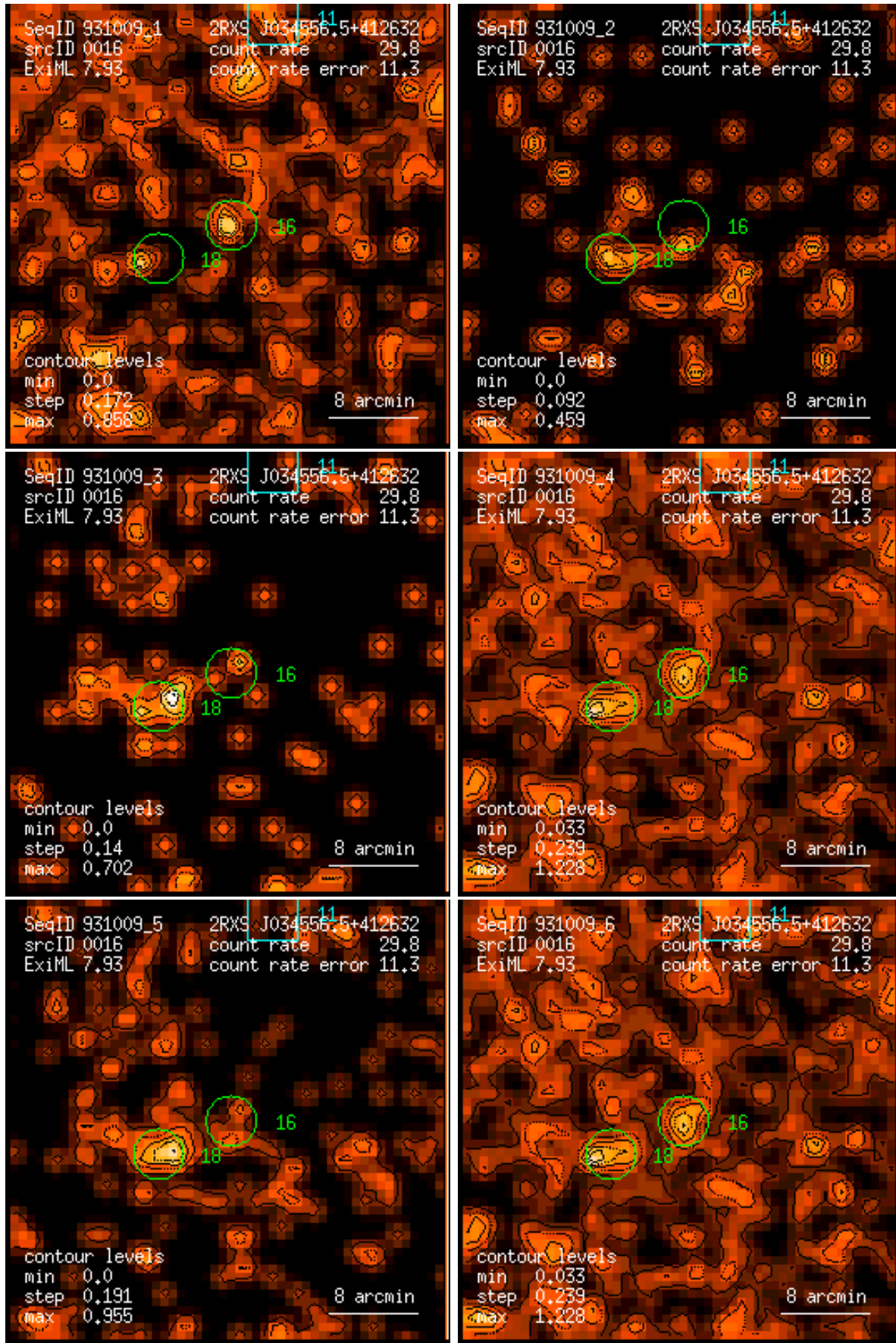
Figure 16: RASS 931009: detection 0016: band rate images, Gaussian filter: (1) PSPC channels 11 – 41, (2) 52 – 90, (3) 91 – 201, (4) 11 – 235, (5) 52 – 201, (6) 11 – 201. Broad band rates in counts/ks. Band rate contour levels in counts/ks/arcmin 2 .
