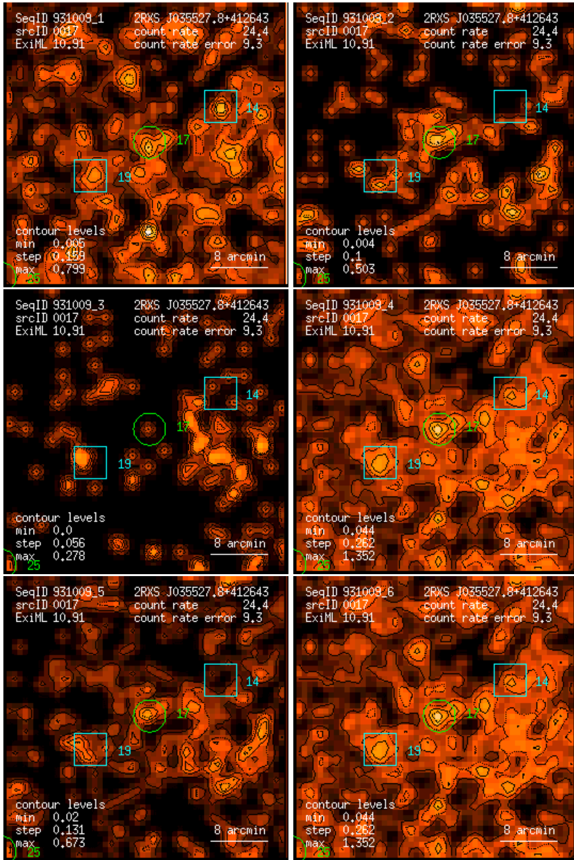
Figure 17: RASS 931009: detection 0017: band rate images, Gaussian filter: (1) PSPC channels 11 – 41, (2) 52 – 90, (3) 91 – 201, (4) 11 – 235, (5) 52 – 201, (6) 11 – 201. Broad band rates in counts/ks. Band rate contour levels in counts/ks/arcmin 2 .
