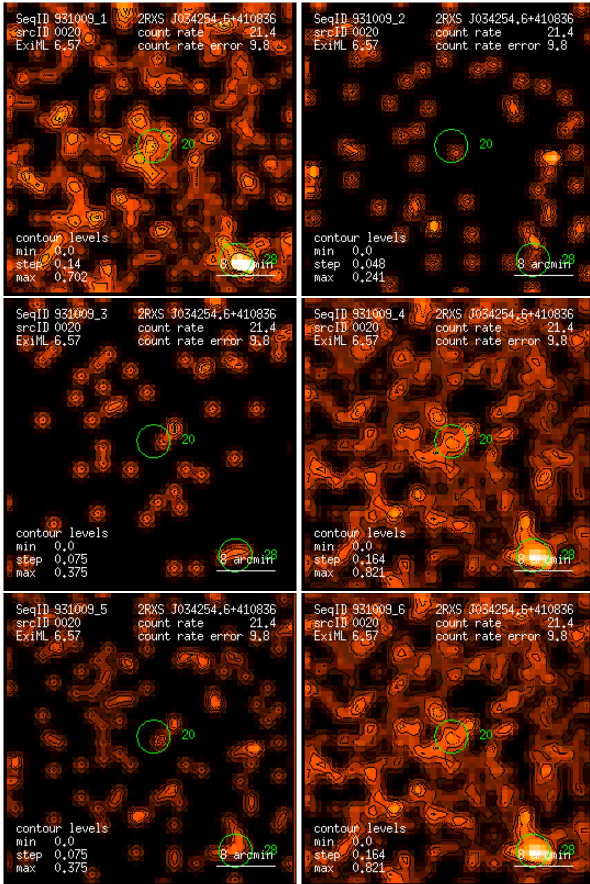
Figure 20: RASS 931009: detection 0020: band rate images, Gaussian filter: (1) PSPC channels 11 – 41, (2) 52 – 90, (3) 91 – 201, (4) 11 – 235, (5) 52 – 201, (6) 11 – 201. Broad band rates in counts/ks. Band rate contour levels in counts/ks/arcmin 2 .
