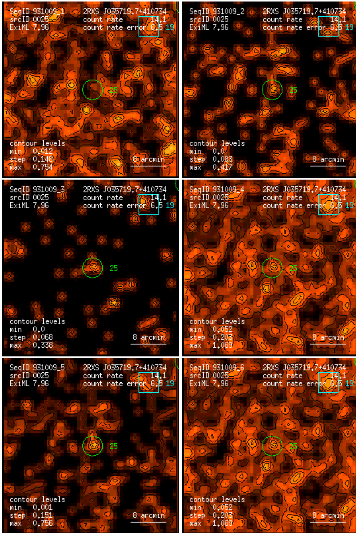
Figure 25: RASS 931009: detection 0025: band rate images, Gaussian filter: (1) PSPC channels 11 – 41, (2) 52 – 90, (3) 91 – 201, (4) 11 – 235, (5) 52 – 201, (6) 11 – 201. Broad band rates in counts/ks. Band rate contour levels in counts/ks/arcmin 2 .
