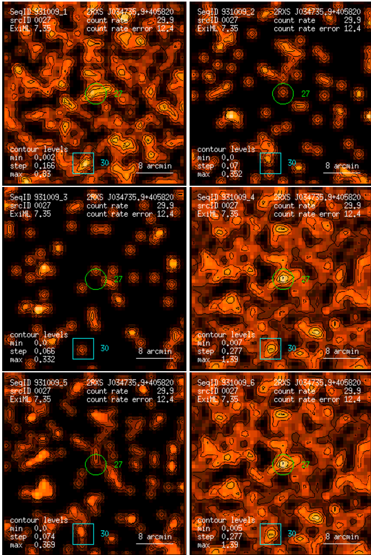
Figure 27: RASS 931009: detection 0027: band rate images, Gaussian filter: (1) PSPC channels 11 – 41, (2) 52 – 90, (3) 91 – 201, (4) 11 – 235, (5) 52 – 201, (6) 11 – 201. Broad band rates in counts/ks. Band rate contour levels in counts/ks/arcmin 2 .
