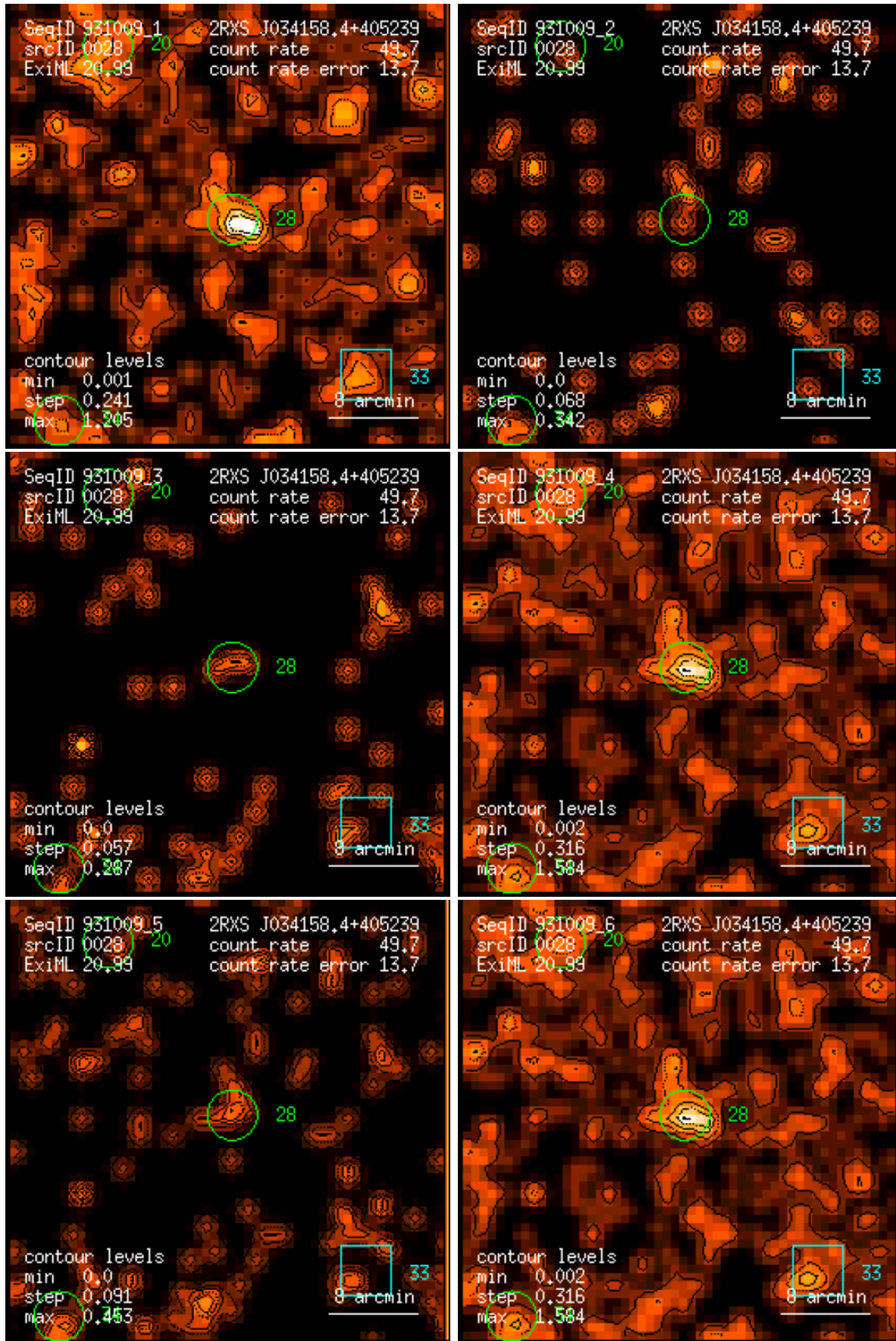
Figure 28: RASS 931009: detection 0028: band rate images, Gaussian filter: (1) PSPC channels 11 – 41, (2) 52 – 90, (3) 91 – 201, (4) 11 – 235, (5) 52 – 201, (6) 11 – 201. Broad band rates in counts/ks. Band rate contour levels in counts/ks/arcmin 2 .
