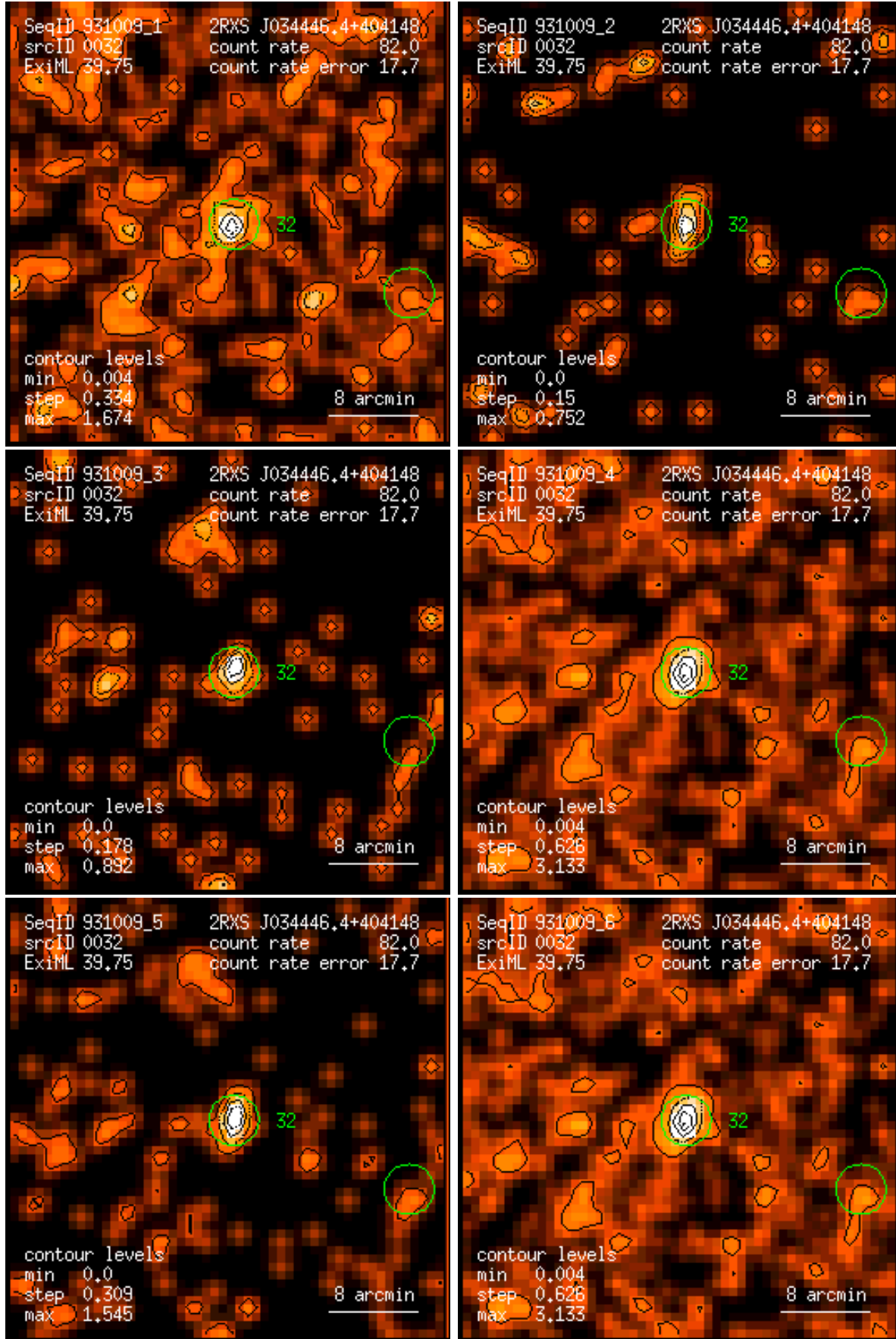
Figure 32: RASS 931009: detection 0032: band rate images, Gaussian filter: (1) PSPC channels 11 – 41, (2) 52 – 90, (3) 91 – 201, (4) 11 – 235, (5) 52 – 201, (6) 11 – 201. Broad band rates in counts/ks. Band rate contour levels in counts/ks/arcmin 2 .
