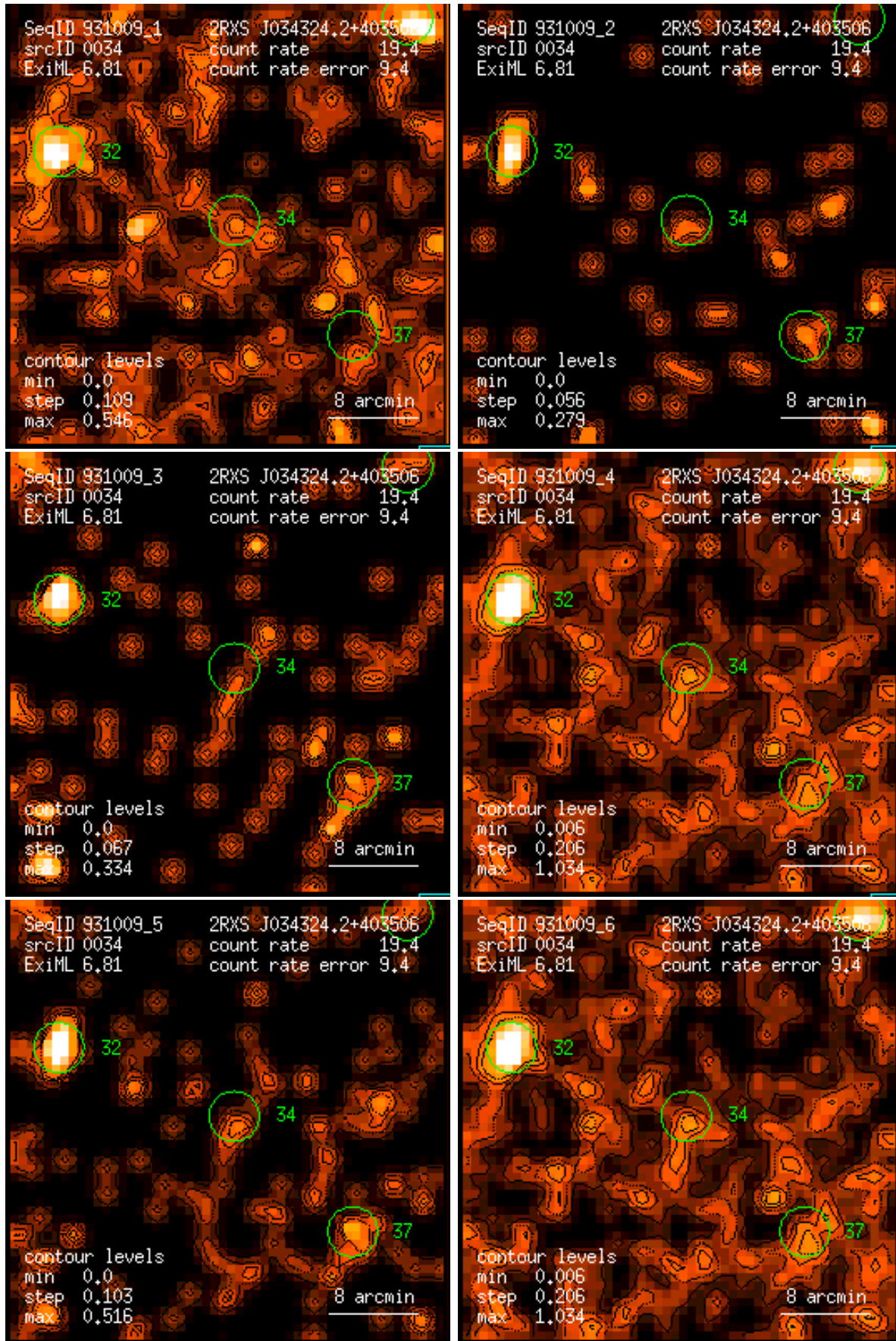
Figure 34: RASS 931009: detection 0034: band rate images, Gaussian filter: (1) PSPC channels 11 – 41, (2) 52 – 90, (3) 91 – 201, (4) 11 – 235, (5) 52 – 201, (6) 11 – 201. Broad band rates in counts/ks. Band rate contour levels in counts/ks/arcmin 2 .
