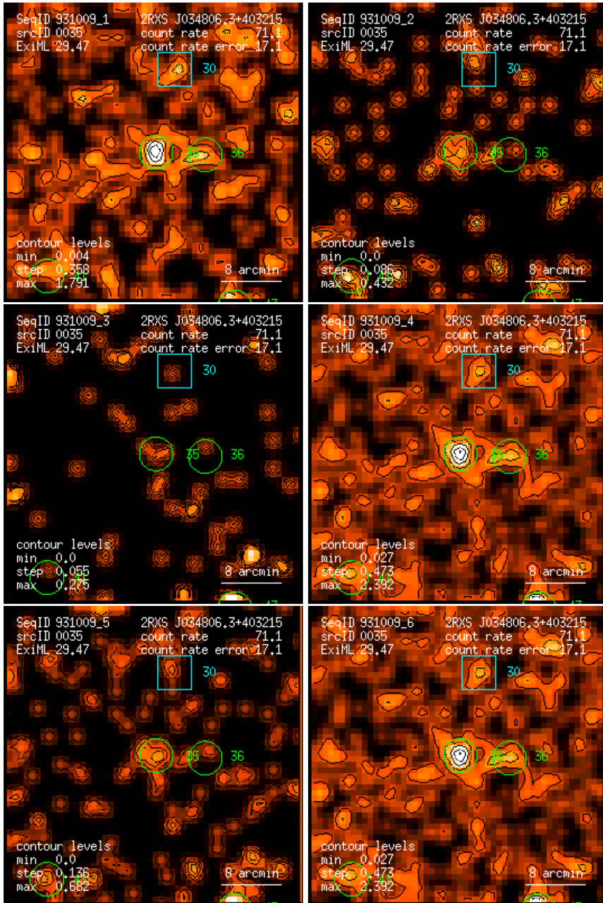
Figure 35: RASS 931009: detection 0035: band rate images, Gaussian filter: (1) PSPC channels 11 – 41, (2) 52 – 90, (3) 91 – 201, (4) 11 – 235, (5) 52 – 201, (6) 11 – 201. Broad band rates in counts/ks. Band rate contour levels in counts/ks/arcmin 2 .
