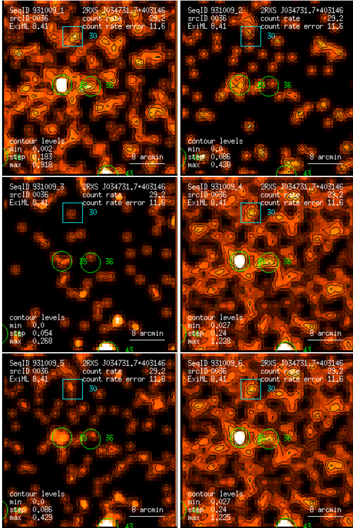
Figure 36: RASS 931009: detection 0036: band rate images, Gaussian filter: (1) PSPC channels 11 – 41, (2) 52 – 90, (3) 91 – 201, (4) 11 – 235, (5) 52 – 201, (6) 11 – 201. Broad band rates in counts/ks. Band rate contour levels in counts/ks/arcmin 2 .
