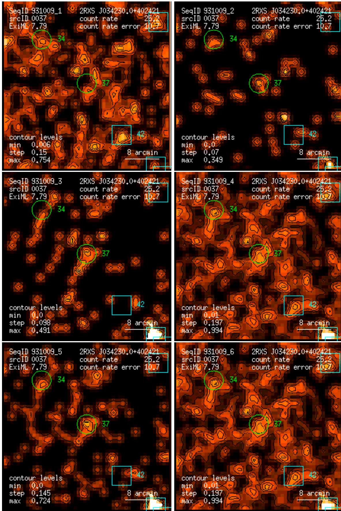
Figure 37: RASS 931009: detection 0037: band rate images, Gaussian filter: (1) PSPC channels 11 – 41, (2) 52 – 90, (3) 91 – 201, (4) 11 – 235, (5) 52 – 201, (6) 11 – 201. Broad band rates in counts/ks. Band rate contour levels in counts/ks/arcmin 2 .
