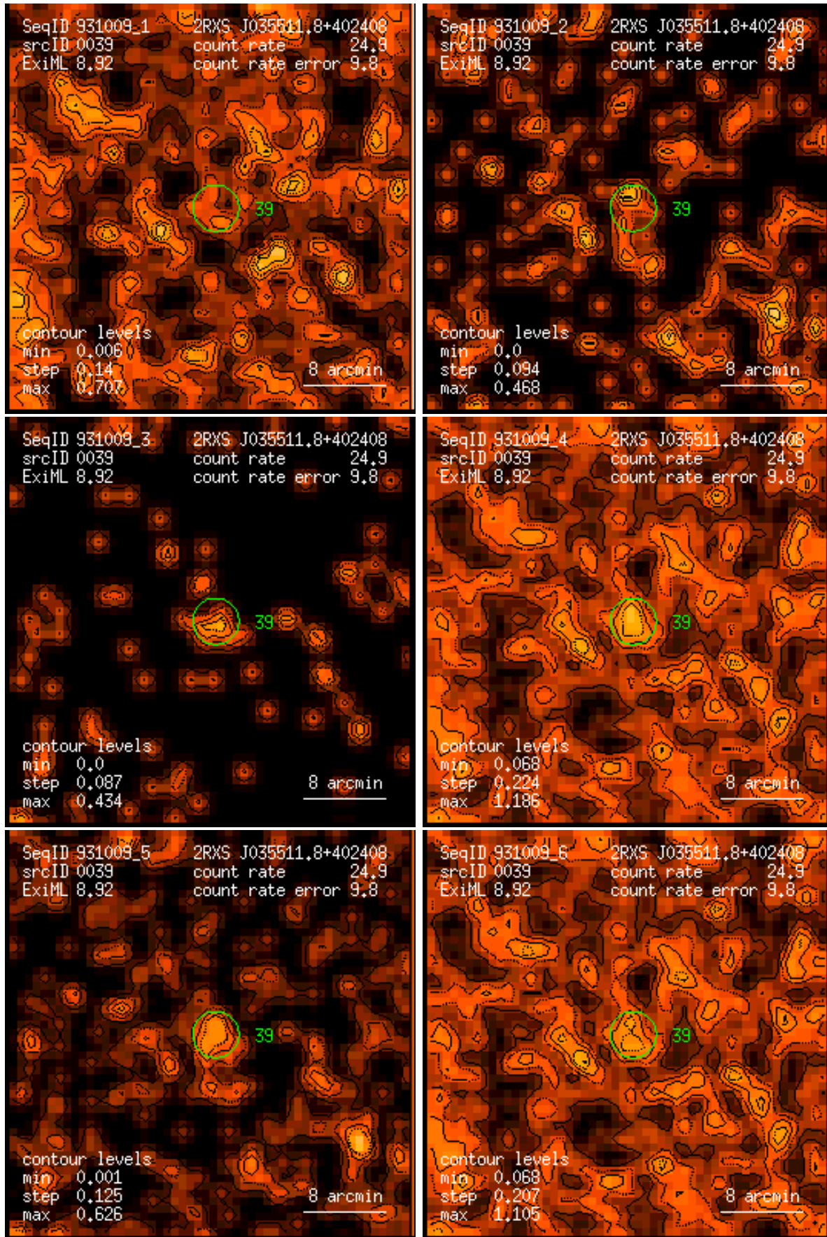
Figure 39: RASS 931009: detection 0039: band rate images, Gaussian filter: (1) PSPC channels 11 – 41, (2) 52 – 90, (3) 91 – 201, (4) 11 – 235, (5) 52 – 201, (6) 11 – 201. Broad band rates in counts/ks. Band rate contour levels in counts/ks/arcmin 2 .
