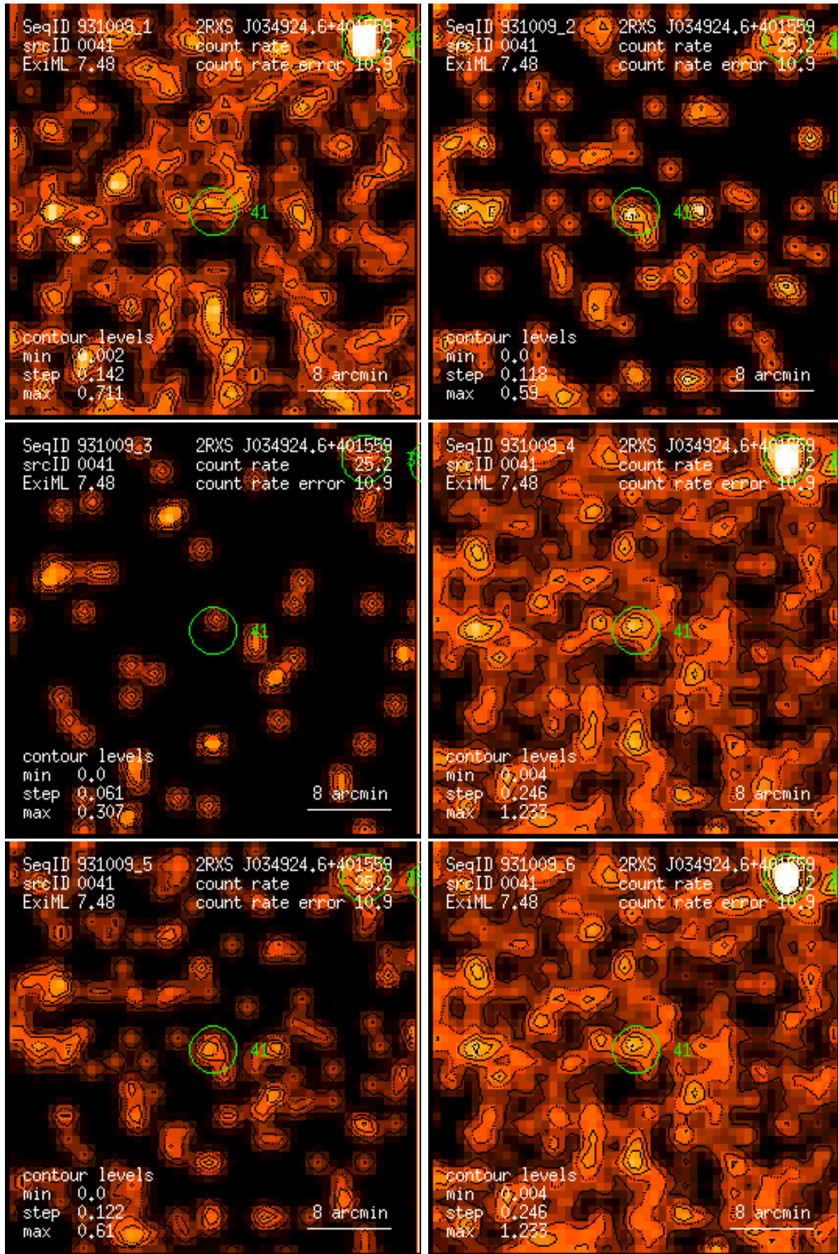
Figure 41: RASS 931009: detection 0041: band rate images, Gaussian filter: (1) PSPC channels 11 – 41, (2) 52 – 90, (3) 91 – 201, (4) 11 – 235, (5) 52 – 201, (6) 11 – 201. Broad band rates in counts/ks. Band rate contour levels in counts/ks/arcmin 2 .
