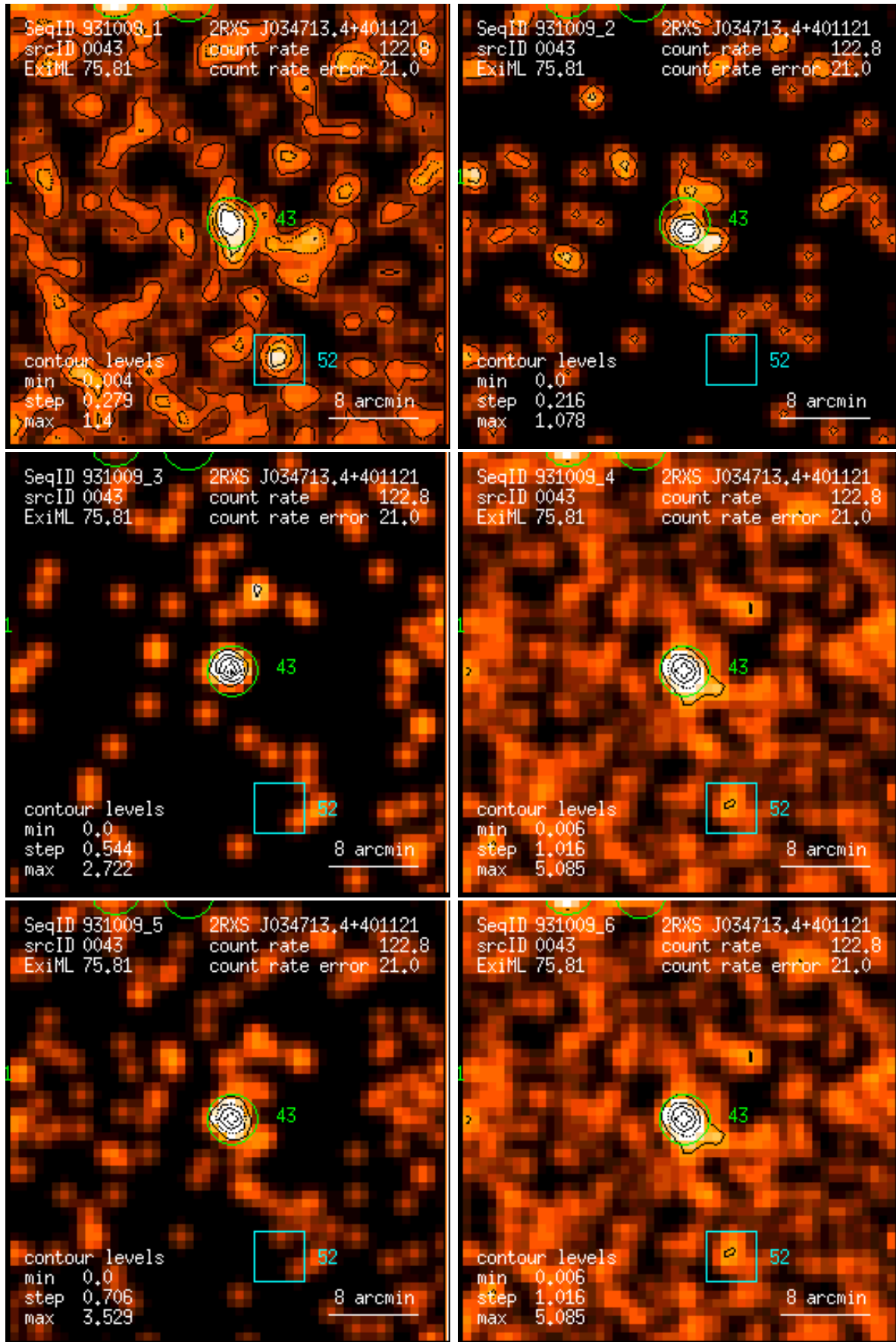
Figure 43: RASS 931009: detection 0043: band rate images, Gaussian filter: (1) PSPC channels 11 – 41, (2) 52 – 90, (3) 91 – 201, (4) 11 – 235, (5) 52 – 201, (6) 11 – 201. Broad band rates in counts/ks. Band rate contour levels in counts/ks/arcmin 2 .
