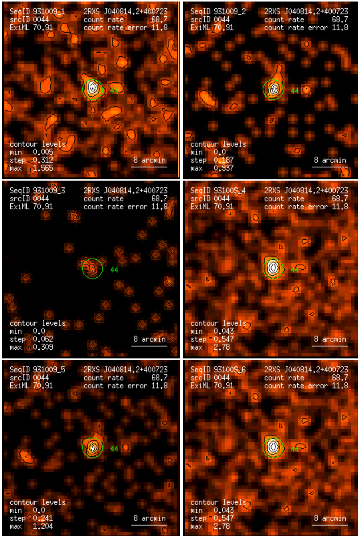
Figure 44: RASS 931009: detection 0044: band rate images, Gaussian filter: (1) PSPC channels 11 – 41, (2) 52 – 90, (3) 91 – 201, (4) 11 – 235, (5) 52 – 201, (6) 11 – 201. Broad band rates in counts/ks. Band rate contour levels in counts/ks/arcmin 2 .
