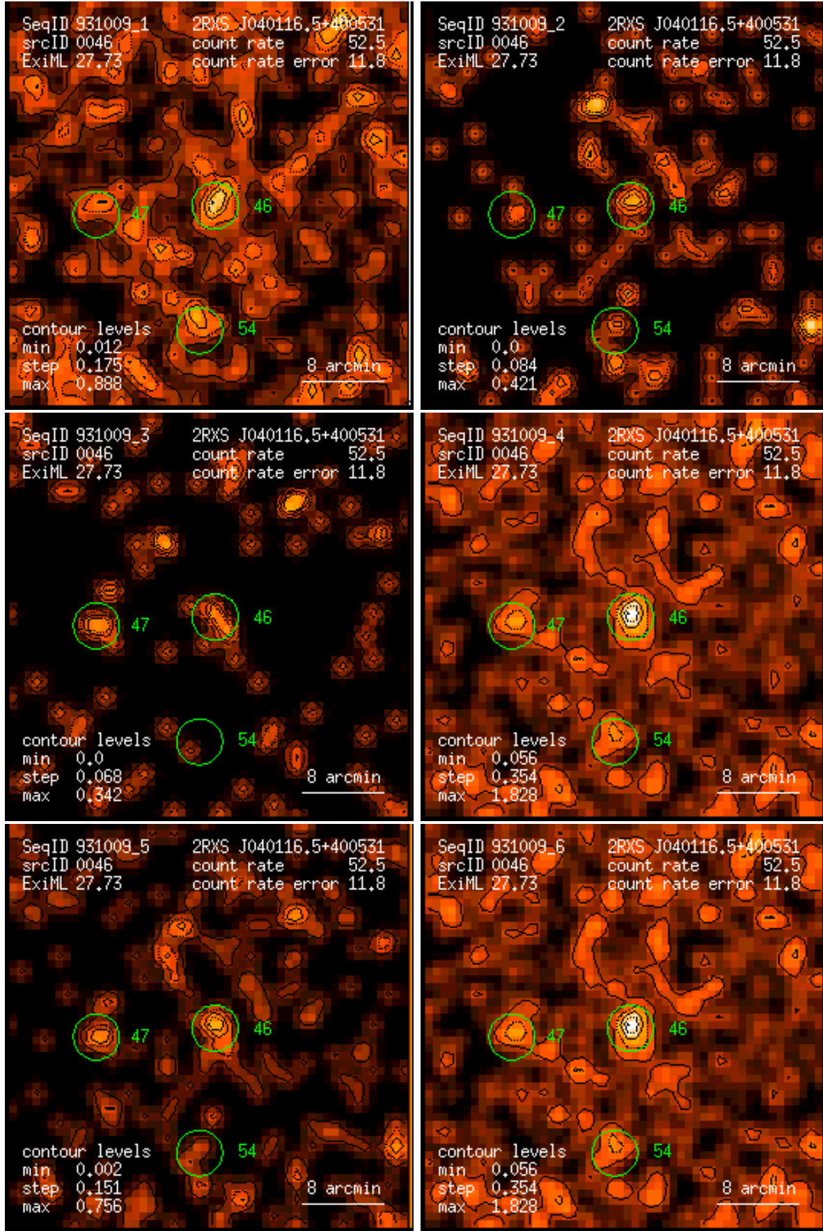
Figure 46: RASS 931009: detection 0046: band rate images, Gaussian filter: (1) PSPC channels 11 – 41, (2) 52 – 90, (3) 91 – 201, (4) 11 – 235, (5) 52 – 201, (6) 11 – 201. Broad band rates in counts/ks. Band rate contour levels in counts/ks/arcmin 2 .
