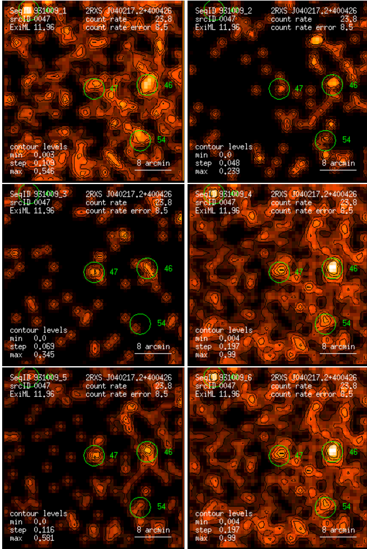
Figure 47: RASS 931009: detection 0047: band rate images, Gaussian filter: (1) PSPC channels 11 – 41, (2) 52 – 90, (3) 91 – 201, (4) 11 – 235, (5) 52 – 201, (6) 11 – 201. Broad band rates in counts/ks. Band rate contour levels in counts/ks/arcmin 2 .
