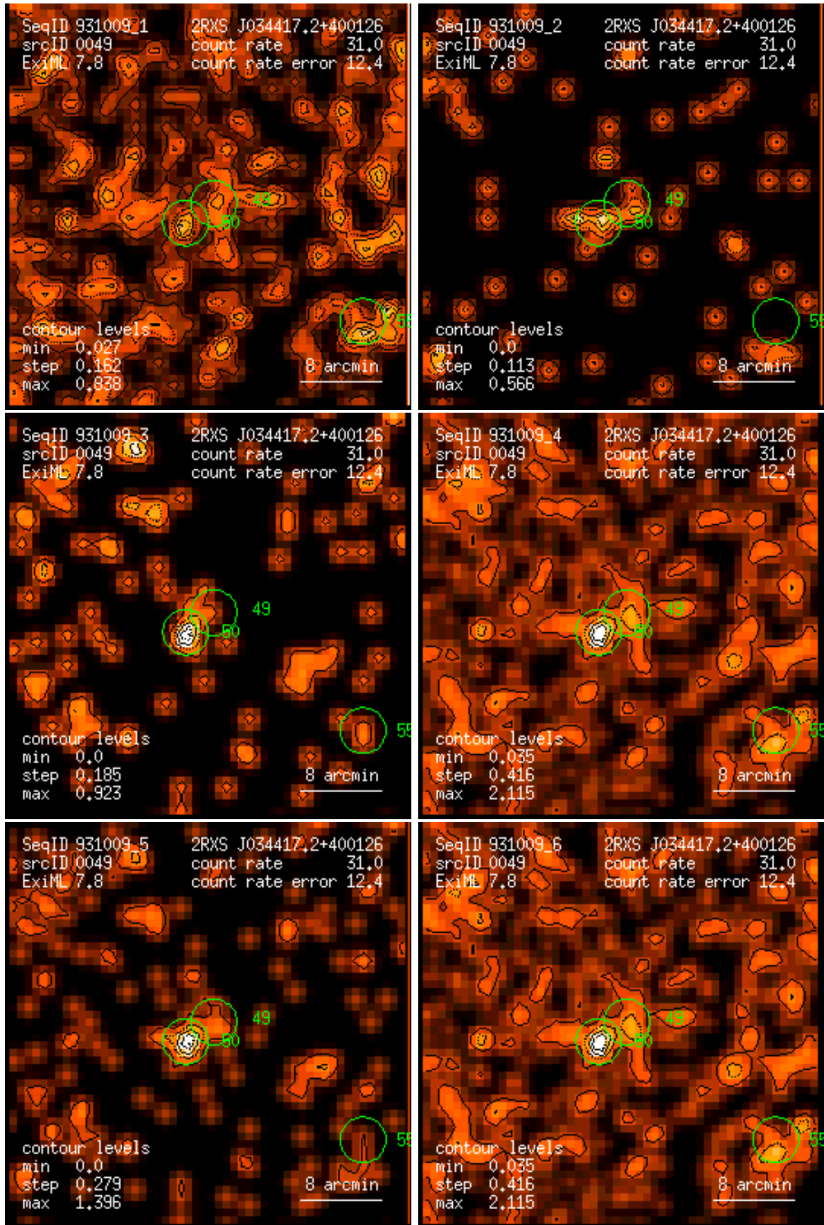
Figure 49: RASS 931009: detection 0049: band rate images, Gaussian filter: (1) PSPC channels 11 – 41, (2) 52 – 90, (3) 91 – 201, (4) 11 – 235, (5) 52 – 201, (6) 11 – 201. Broad band rates in counts/ks. Band rate contour levels in counts/ks/arcmin 2 .
