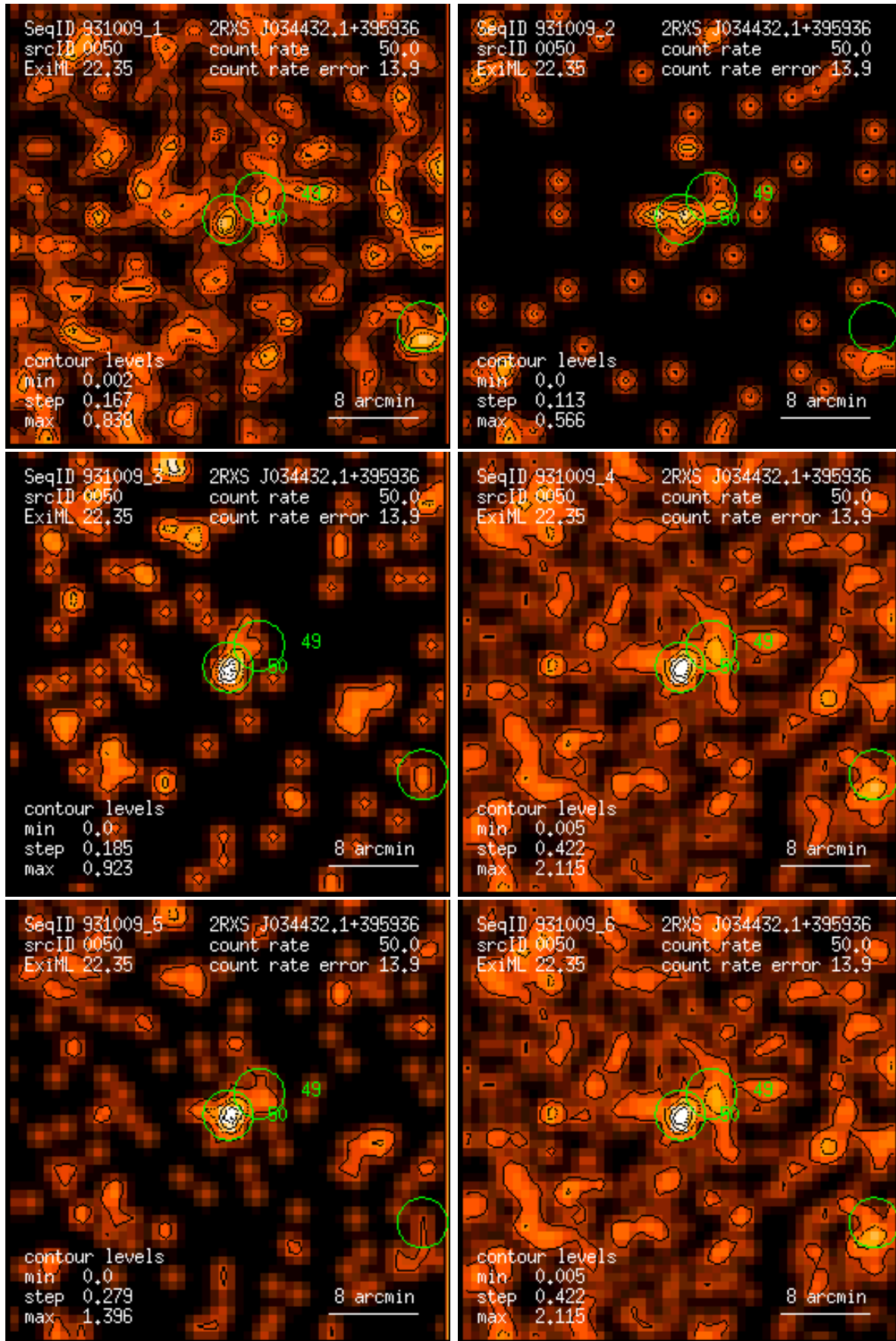
Figure 50: RASS 931009: detection 0050: band rate images, Gaussian filter: (1) PSPC channels 11 – 41, (2) 52 – 90, (3) 91 – 201, (4) 11 – 235, (5) 52 – 201, (6) 11 – 201. Broad band rates in counts/ks. Band rate contour levels in counts/ks/arcmin 2 .
