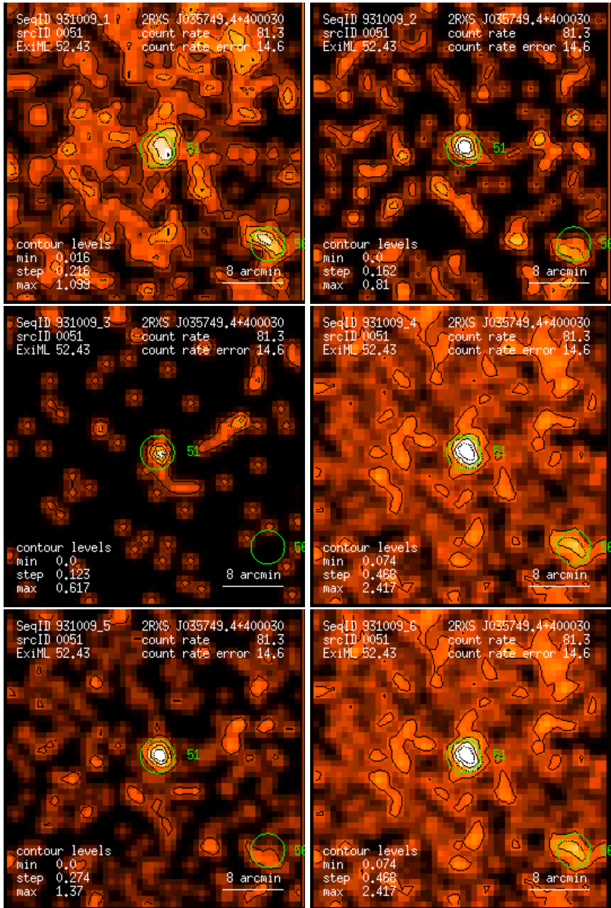
Figure 51: RASS 931009: detection 0051: band rate images, Gaussian filter: (1) PSPC channels 11 – 41, (2) 52 – 90, (3) 91 – 201, (4) 11 – 235, (5) 52 – 201, (6) 11 – 201. Broad band rates in counts/ks. Band rate contour levels in counts/ks/arcmin 2 .
