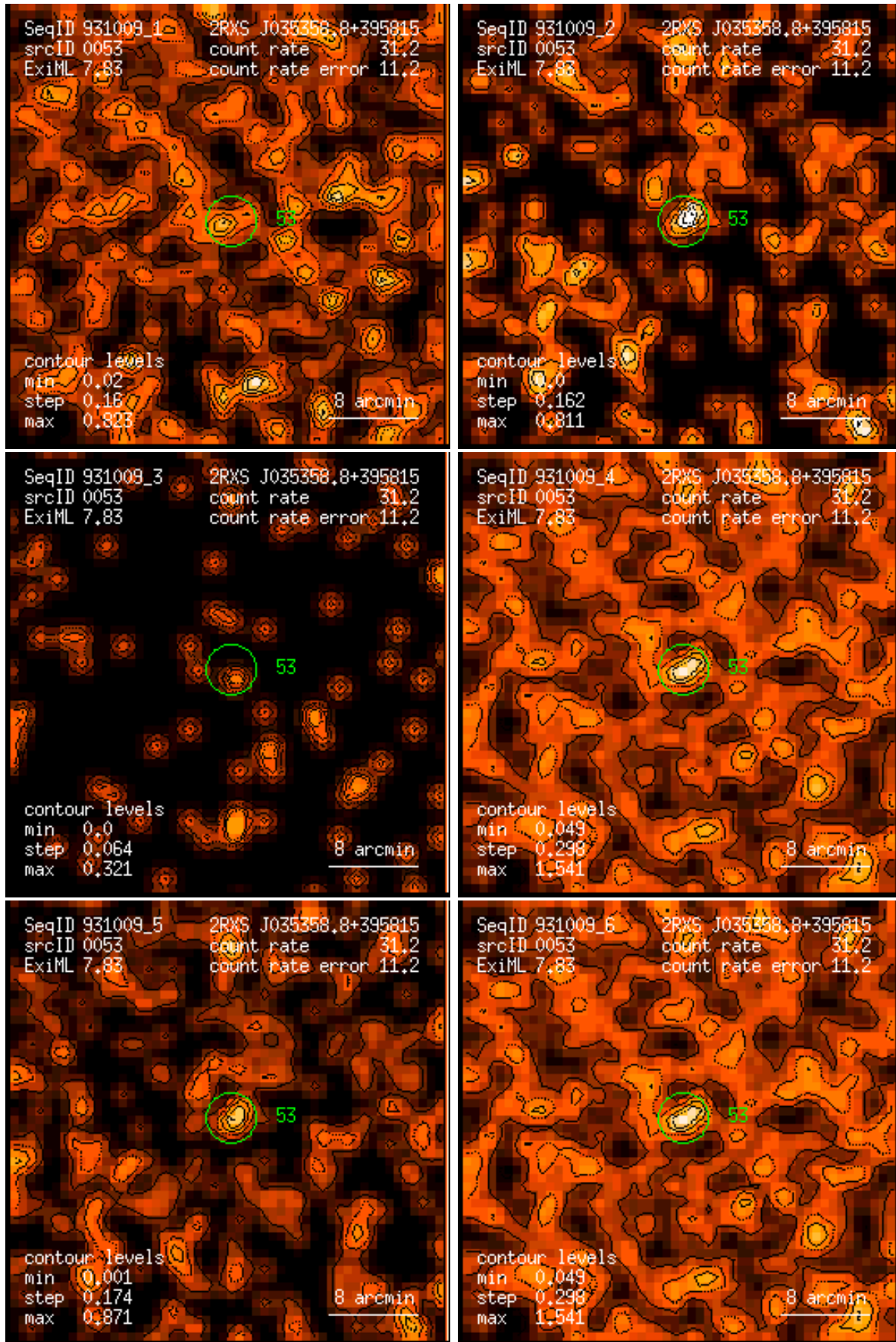
Figure 53: RASS 931009: detection 0053: band rate images, Gaussian filter: (1) PSPC channels 11 – 41, (2) 52 – 90, (3) 91 – 201, (4) 11 – 235, (5) 52 – 201, (6) 11 – 201. Broad band rates in counts/ks. Band rate contour levels in counts/ks/arcmin 2 .
