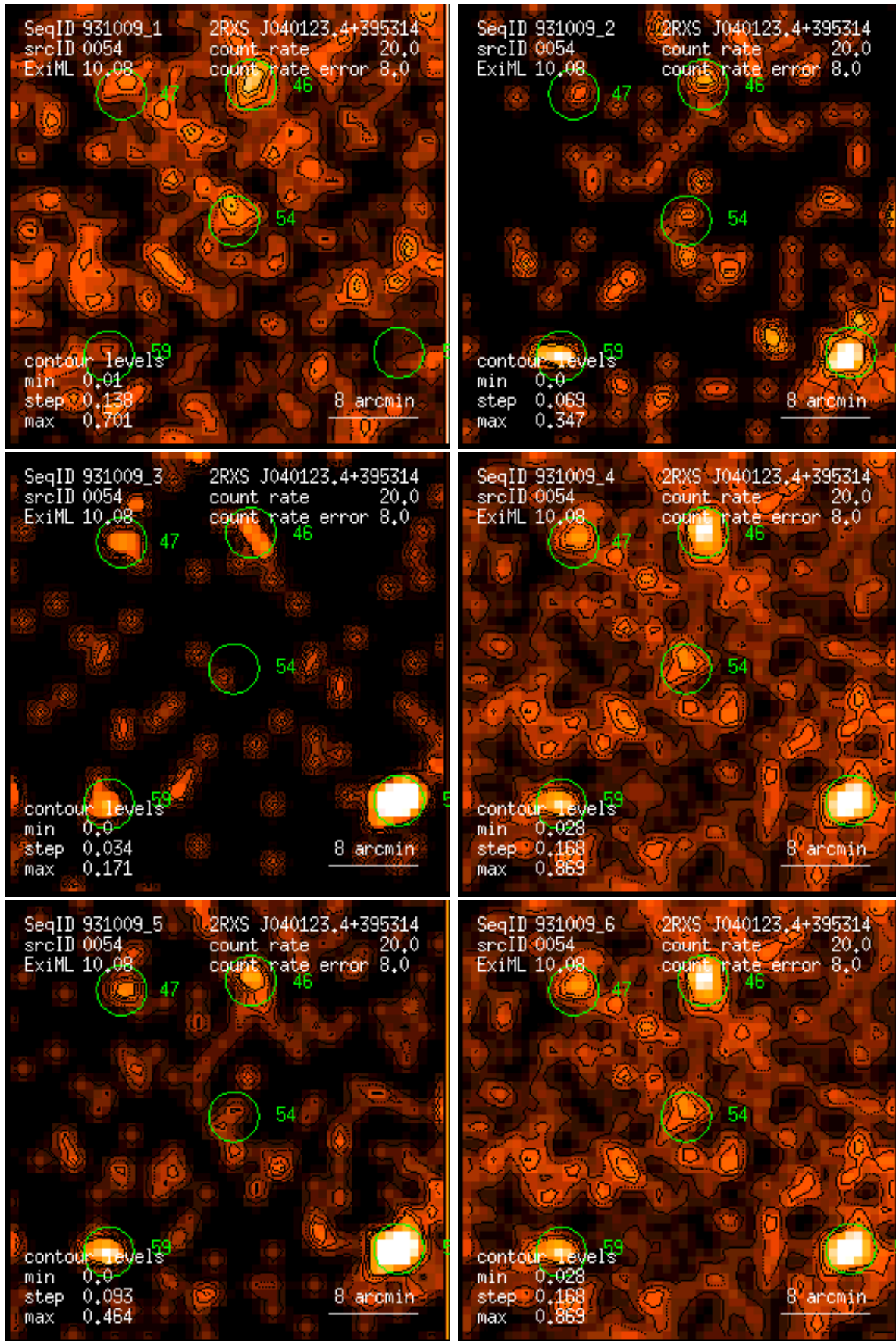
Figure 54: RASS 931009: detection 0054: band rate images, Gaussian filter: (1) PSPC channels 11 – 41, (2) 52 – 90, (3) 91 – 201, (4) 11 – 235, (5) 52 – 201, (6) 11 – 201. Broad band rates in counts/ks. Band rate contour levels in counts/ks/arcmin 2 .
