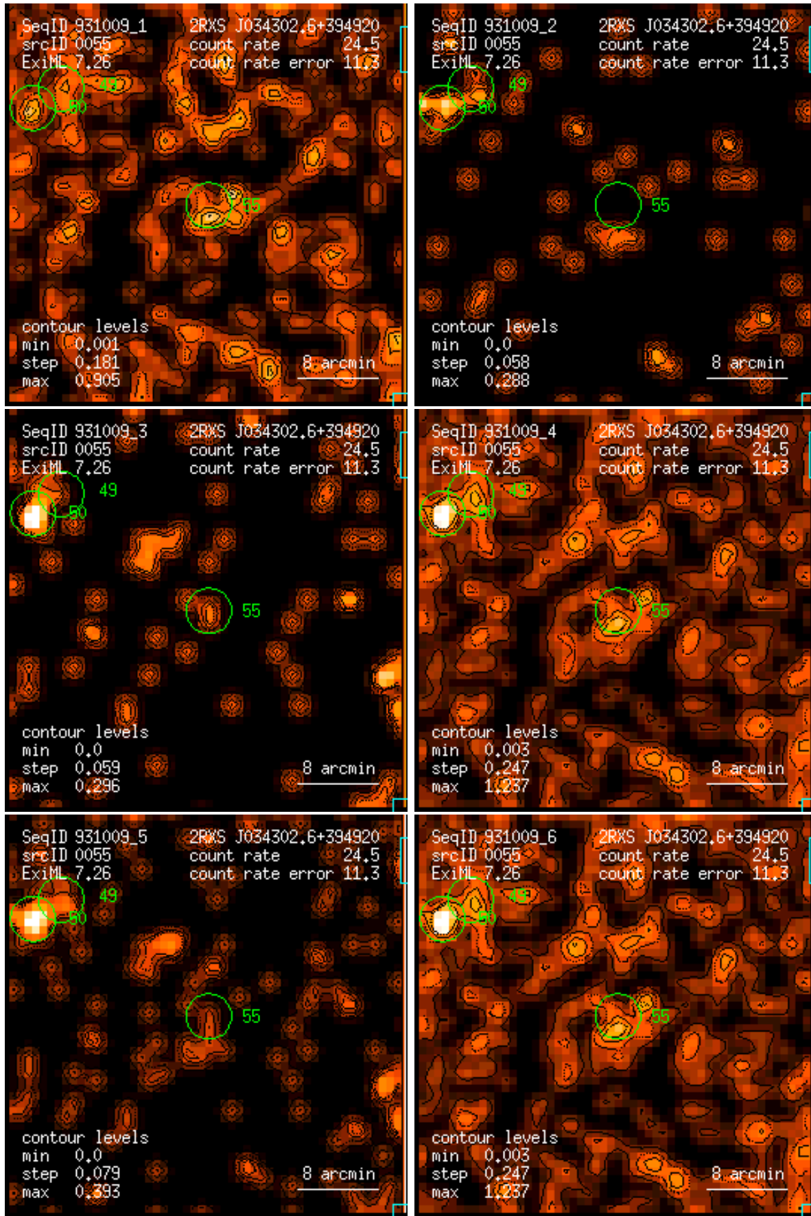
Figure 55: RASS 931009: detection 0055: band rate images, Gaussian filter: (1) PSPC channels 11 – 41, (2) 52 – 90, (3) 91 – 201, (4) 11 – 235, (5) 52 – 201, (6) 11 – 201. Broad band rates in counts/ks. Band rate contour levels in counts/ks/arcmin 2 .
