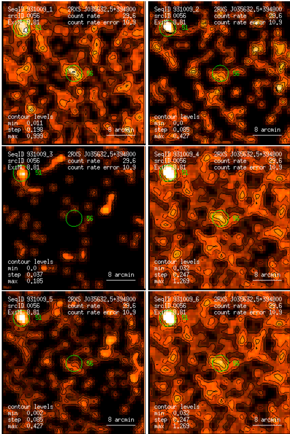
Figure 56: RASS 931009: detection 0056: band rate images, Gaussian filter: (1) PSPC channels 11 – 41, (2) 52 – 90, (3) 91 – 201, (4) 11 – 235, (5) 52 – 201, (6) 11 – 201. Broad band rates in counts/ks. Band rate contour levels in counts/ks/arcmin 2 .
