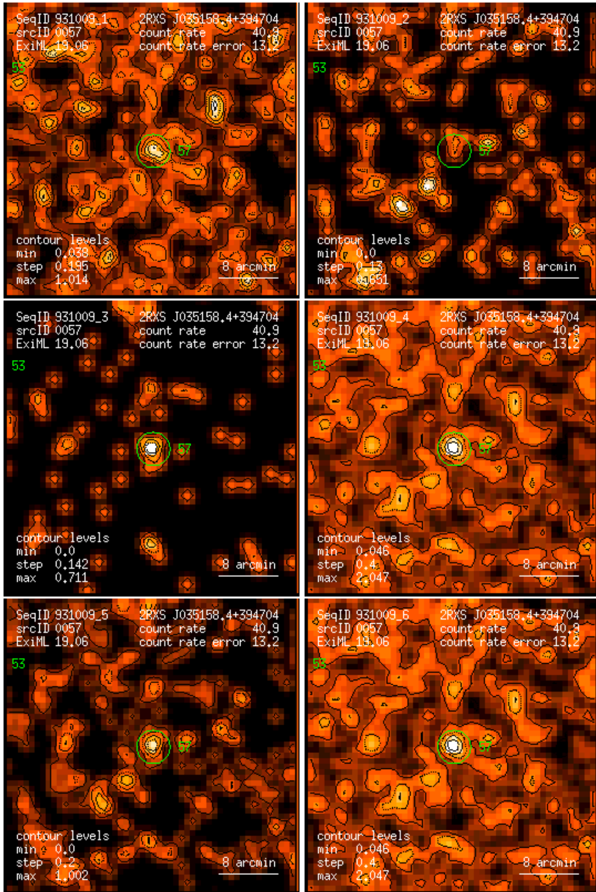
Figure 57: RASS 931009: detection 0057: band rate images, Gaussian filter: (1) PSPC channels 11 – 41, (2) 52 – 90, (3) 91 – 201, (4) 11 – 235, (5) 52 – 201, (6) 11 – 201. Broad band rates in counts/ks. Band rate contour levels in counts/ks/arcmin 2 .
