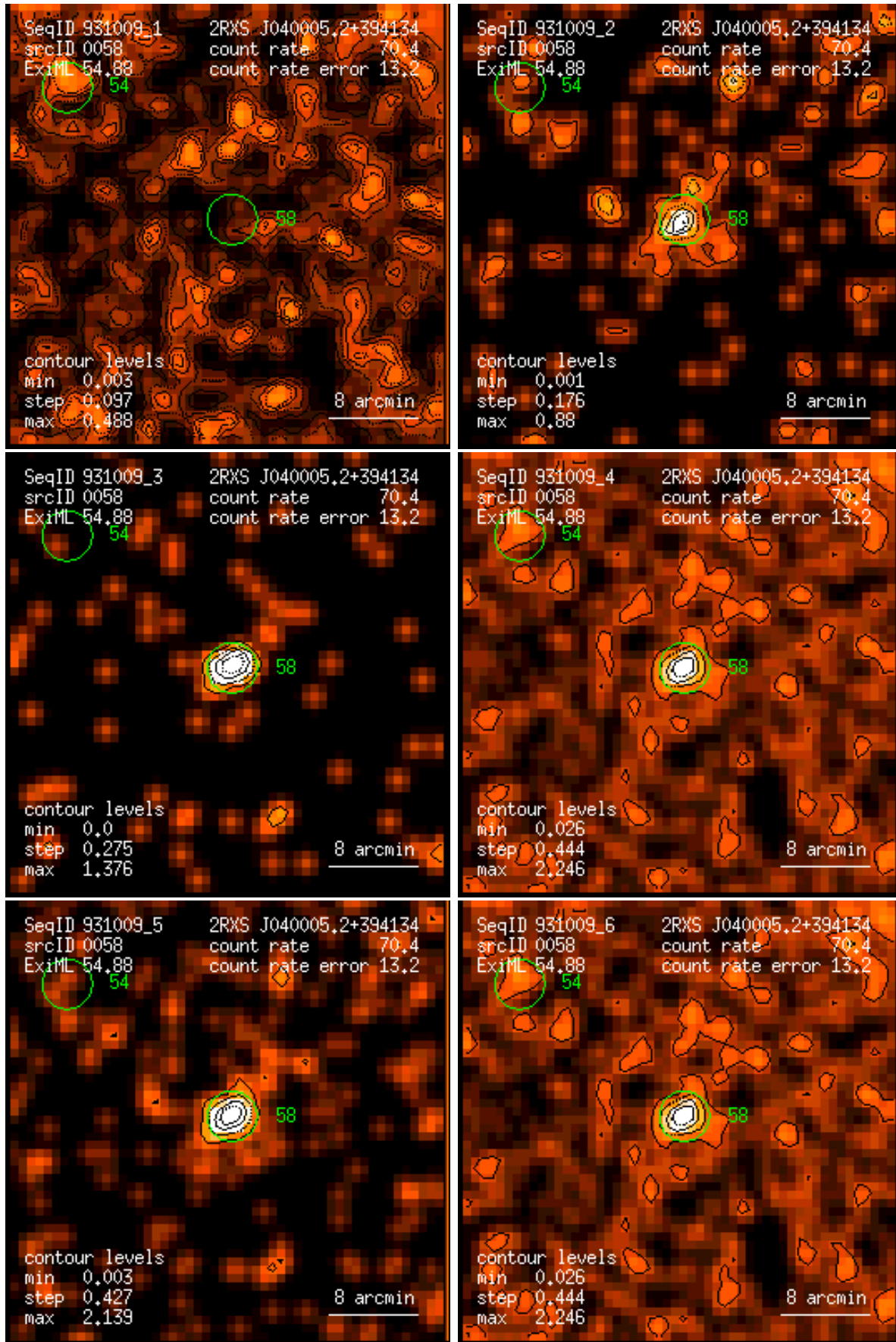
Figure 58: RASS 931009: detection 0058: band rate images, Gaussian filter: (1) PSPC channels 11 – 41, (2) 52 – 90, (3) 91 – 201, (4) 11 – 235, (5) 52 – 201, (6) 11 – 201. Broad band rates in counts/ks. Band rate contour levels in counts/ks/arcmin 2 .
