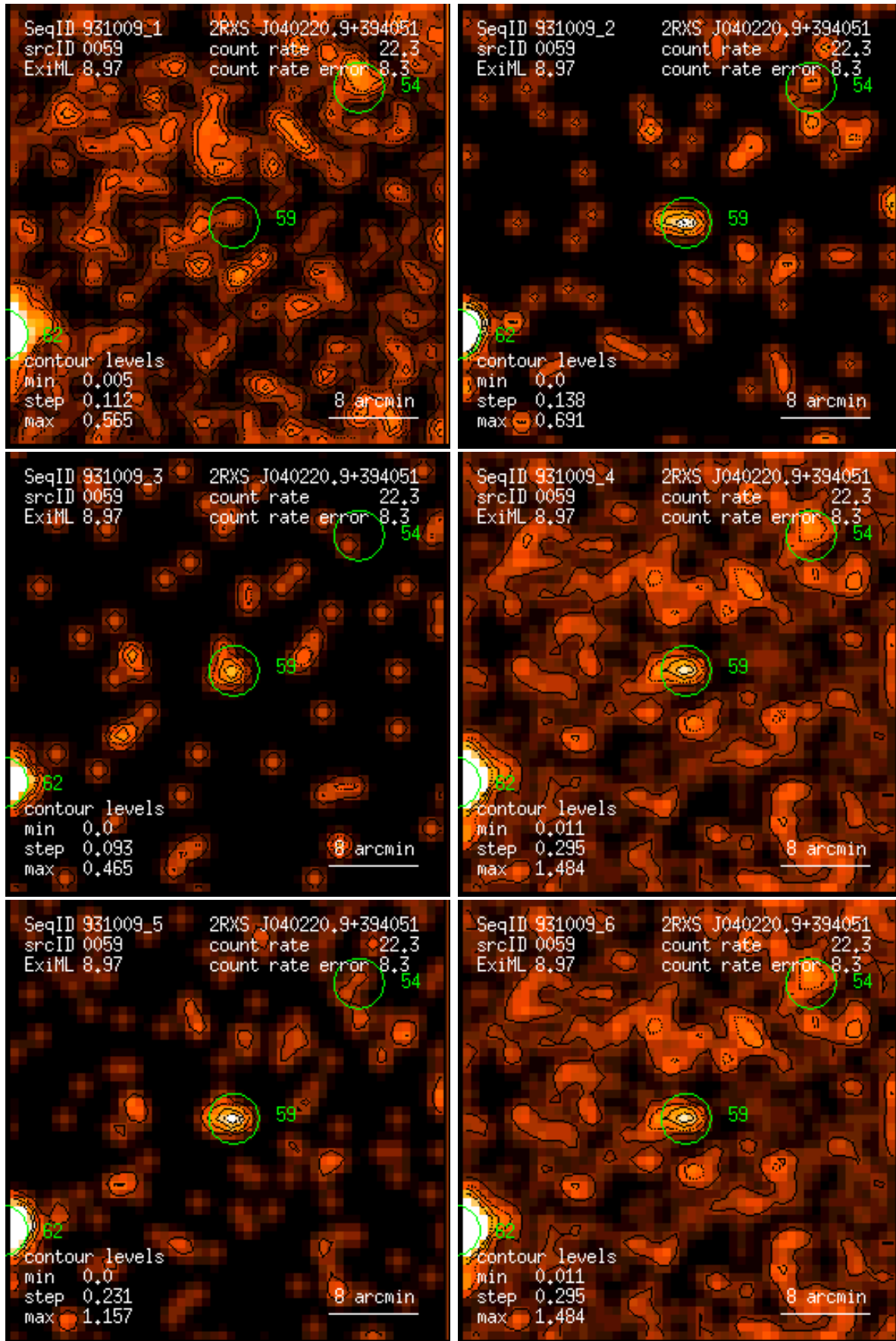
Figure 59: RASS 931009: detection 0059: band rate images, Gaussian filter: (1) PSPC channels 11 – 41, (2) 52 – 90, (3) 91 – 201, (4) 11 – 235, (5) 52 – 201, (6) 11 – 201. Broad band rates in counts/ks. Band rate contour levels in counts/ks/arcmin 2 .
