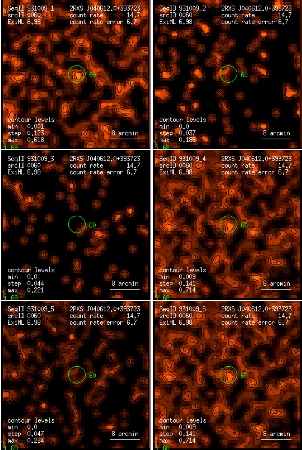
Figure 60: RASS 931009: detection 0060: band rate images, Gaussian filter: (1) PSPC channels 11 – 41, (2) 52 – 90, (3) 91 – 201, (4) 11 – 235, (5) 52 – 201, (6) 11 – 201. Broad band rates in counts/ks. Band rate contour levels in counts/ks/arcmin 2 .
