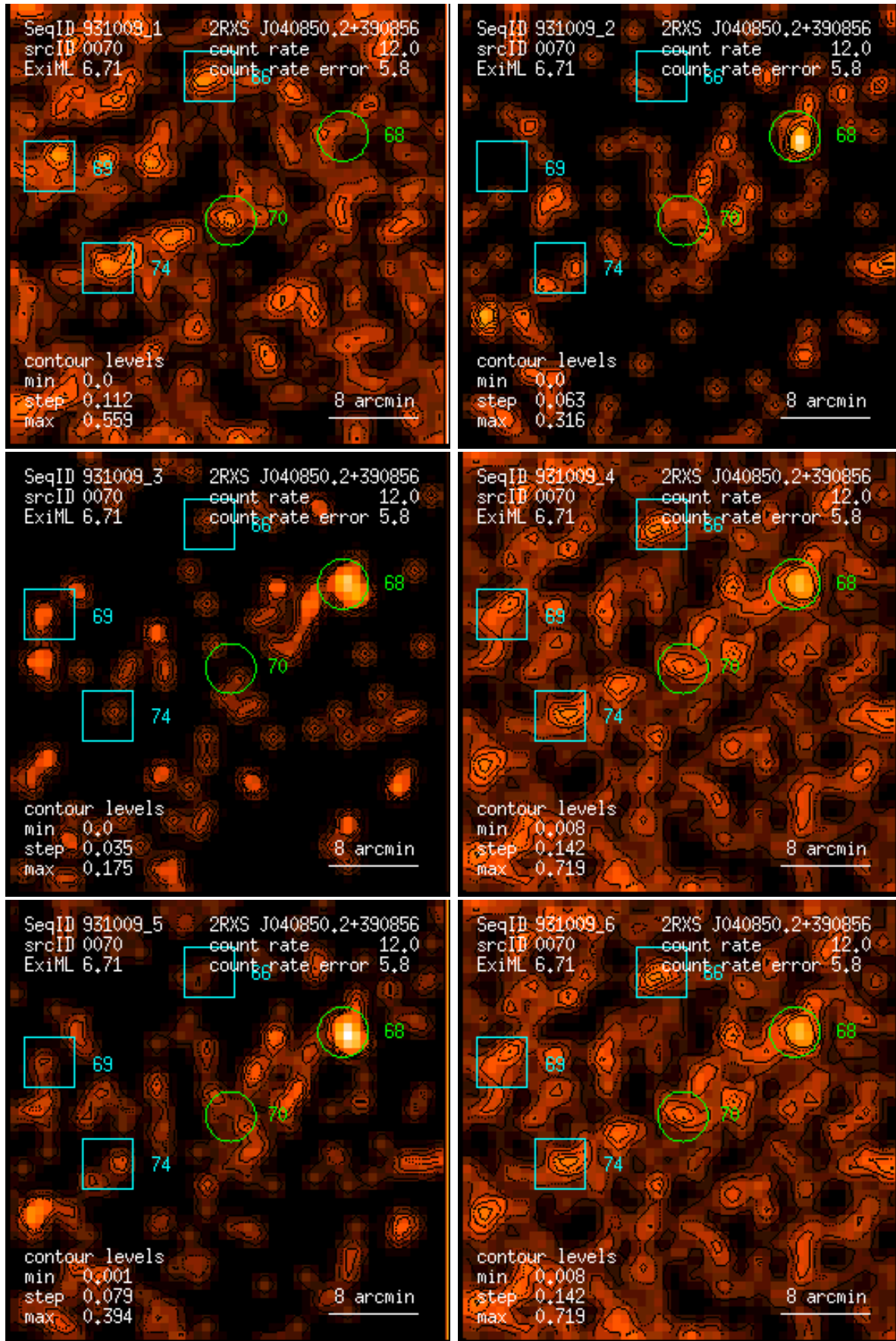
Figure 70: RASS 931009: detection 0070: band rate images, Gaussian filter: (1) PSPC channels 11 – 41, (2) 52 – 90, (3) 91 – 201, (4) 11 – 235, (5) 52 – 201, (6) 11 – 201. Broad band rates in counts/ks. Band rate contour levels in counts/ks/arcmin 2 .
