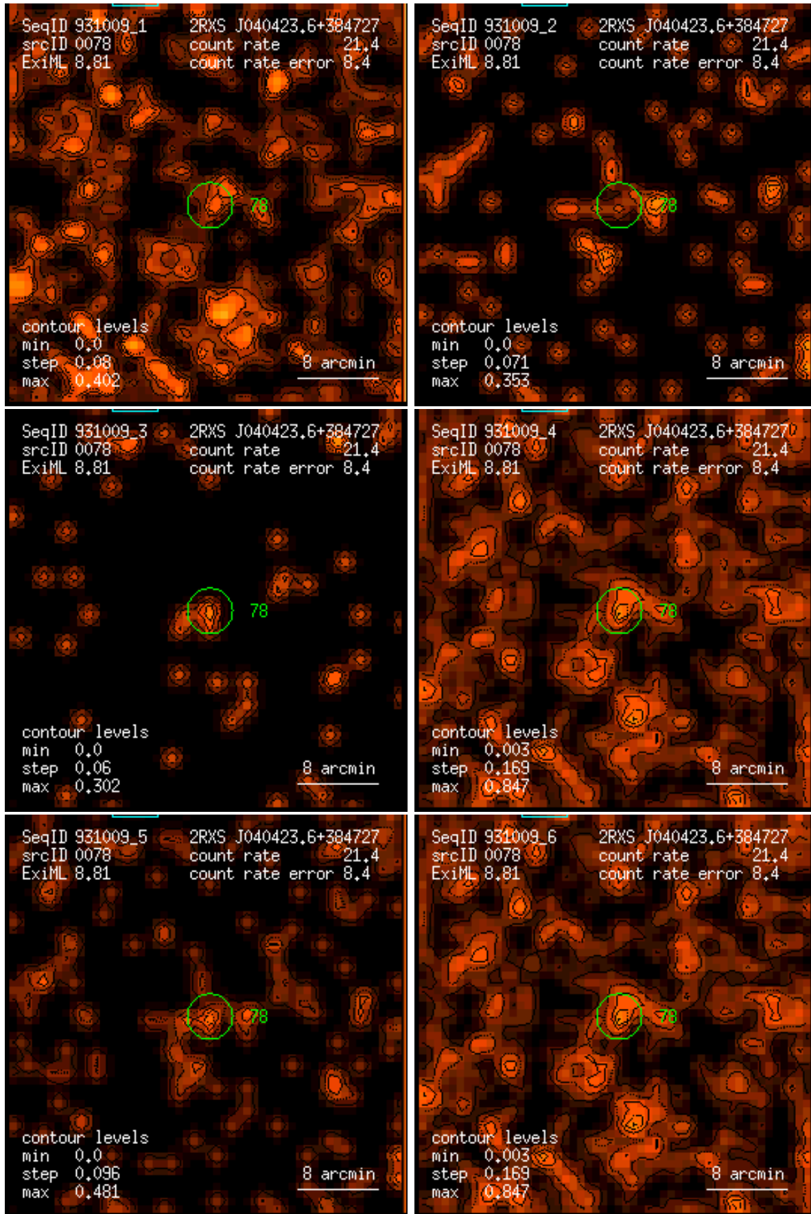
Figure 78: RASS 931009: detection 0078: band rate images, Gaussian filter: (1) PSPC channels 11 – 41, (2) 52 – 90, (3) 91 – 201, (4) 11 – 235, (5) 52 – 201, (6) 11 – 201. Broad band rates in counts/ks. Band rate contour levels in counts/ks/arcmin 2 .
