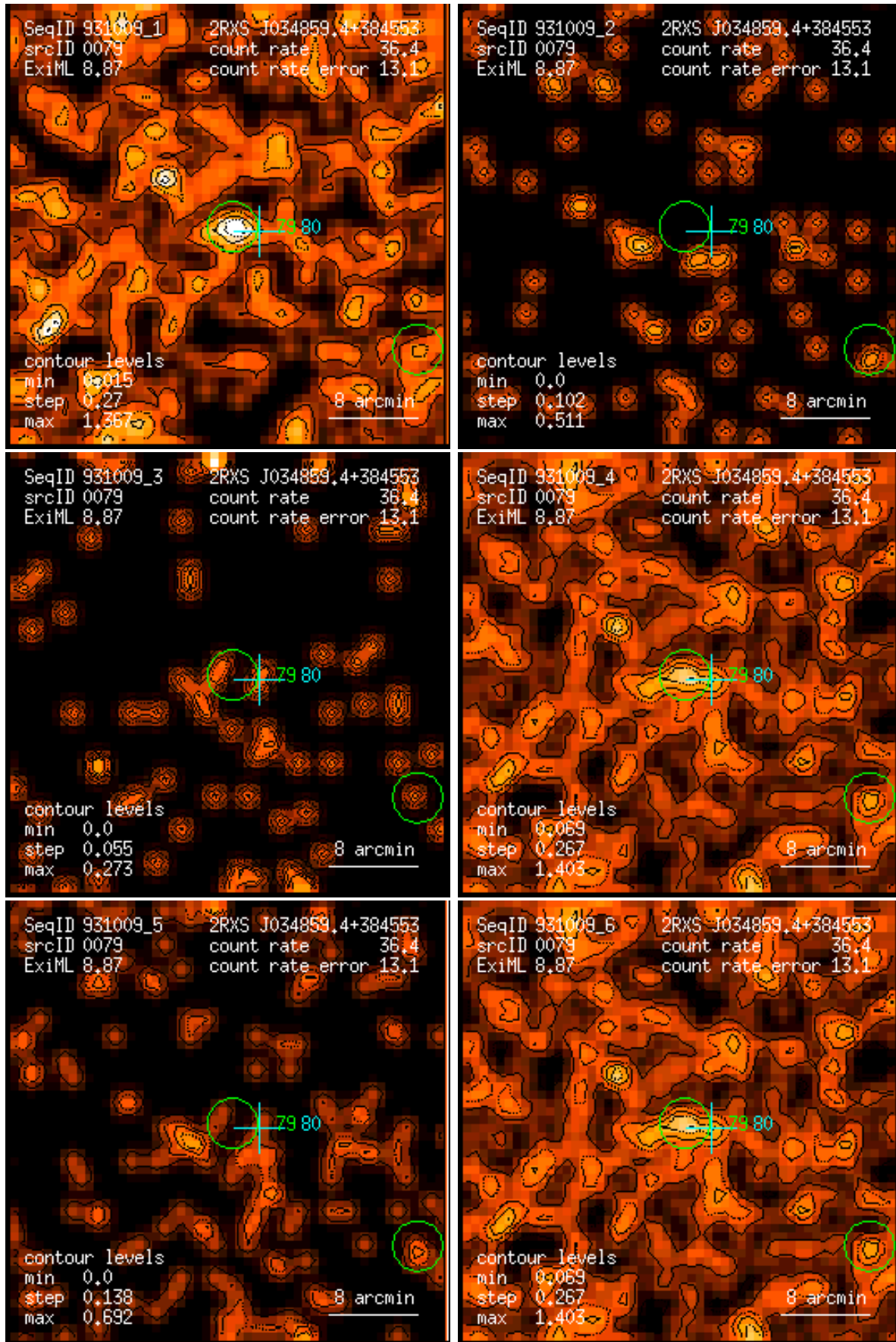
Figure 79: RASS 931009: detection 0079: band rate images, Gaussian filter: (1) PSPC channels 11 – 41, (2) 52 – 90, (3) 91 – 201, (4) 11 – 235, (5) 52 – 201, (6) 11 – 201. Broad band rates in counts/ks. Band rate contour levels in counts/ks/arcmin 2 .
