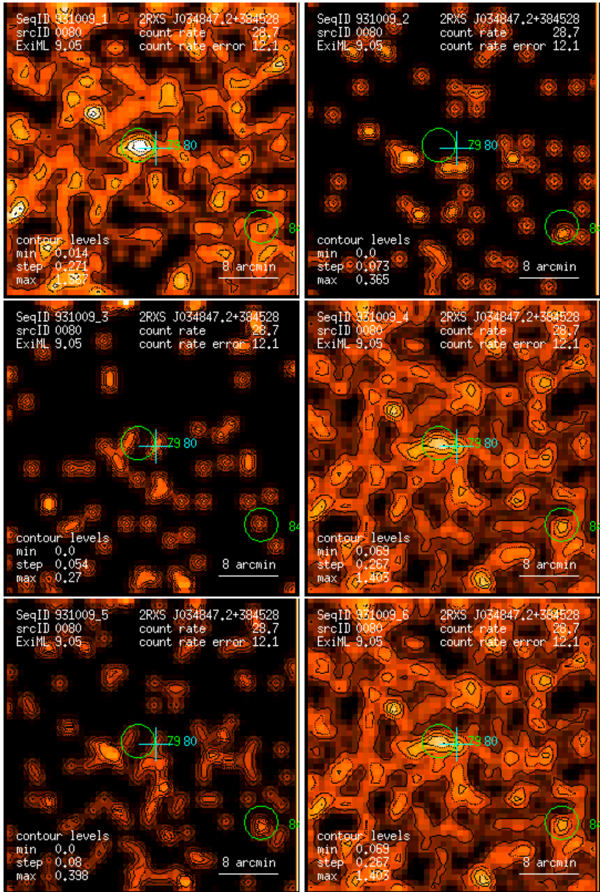
Figure 80: RASS 931009: detection 0080: band rate images, Gaussian filter: (1) PSPC channels 11 – 41, (2) 52 – 90, (3) 91 – 201, (4) 11 – 235, (5) 52 – 201, (6) 11 – 201. Broad band rates in counts/ks. Band rate contour levels in counts/ks/arcmin 2 .
