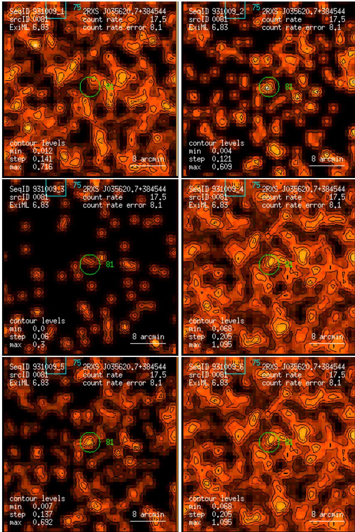
Figure 81: RASS 931009: detection 0081: band rate images, Gaussian filter: (1) PSPC channels 11 – 41, (2) 52 – 90, (3) 91 – 201, (4) 11 – 235, (5) 52 – 201, (6) 11 – 201. Broad band rates in counts/ks. Band rate contour levels in counts/ks/arcmin 2 .
