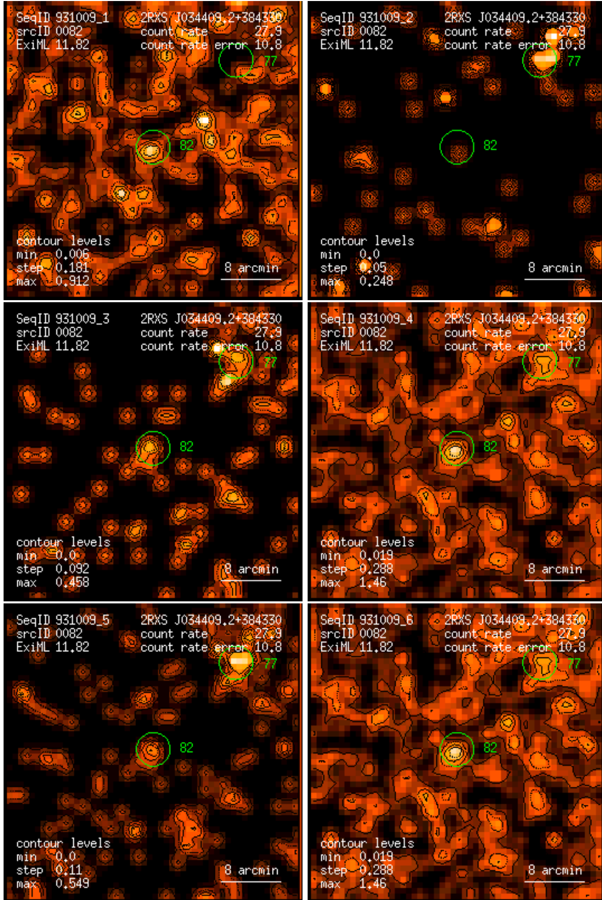
Figure 82: RASS 931009: detection 0082: band rate images, Gaussian filter: (1) PSPC channels 11 – 41, (2) 52 – 90, (3) 91 – 201, (4) 11 – 235, (5) 52 – 201, (6) 11 – 201. Broad band rates in counts/ks. Band rate contour levels in counts/ks/arcmin 2 .
