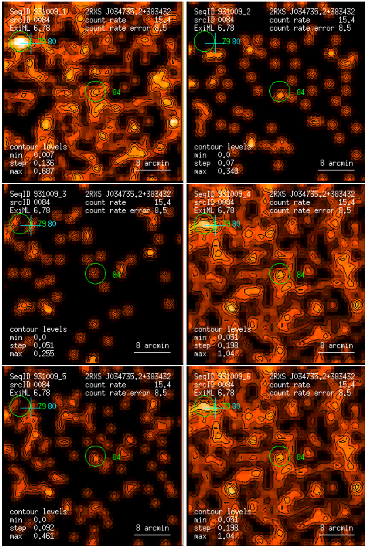
Figure 84: RASS 931009: detection 0084: band rate images, Gaussian filter: (1) PSPC channels 11 – 41, (2) 52 – 90, (3) 91 – 201, (4) 11 – 235, (5) 52 – 201, (6) 11 – 201. Broad band rates in counts/ks. Band rate contour levels in counts/ks/arcmin 2 .
